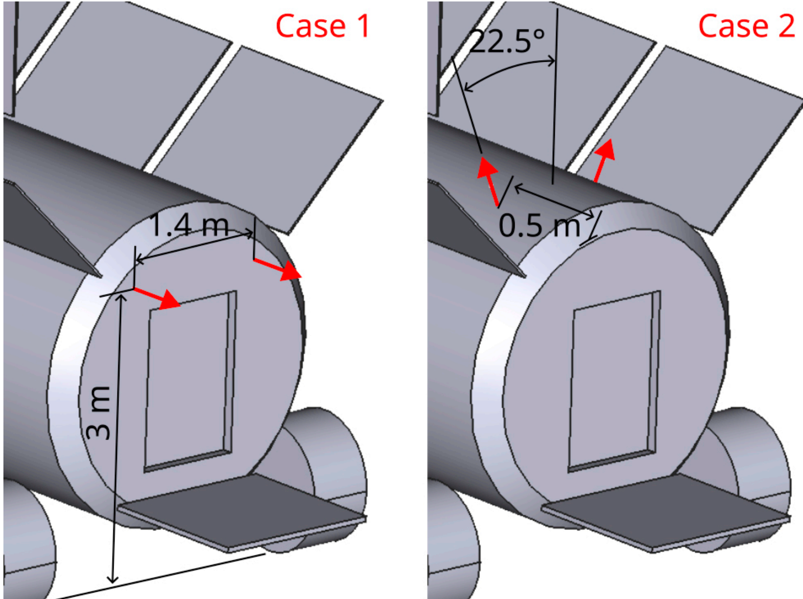
Figure 3. from S. Boccelli et al 2026 Planet. Sci. J. 7 doi:10.3847/PSJ/ae63c4 https://dx.doi.org/10.3847/PSJ/ae63c4 © 2026. The Author(s). Published by the American Astronomical Society.
