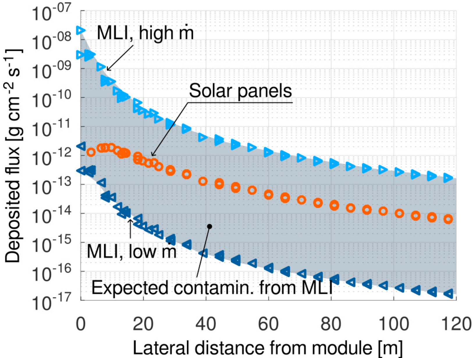
Figure 11. from S. Boccelli et al 2026 Planet. Sci. J. 7 doi:10.3847/PSJ/ae63c4 https://dx.doi.org/10.3847/PSJ/ae63c4 © 2026. The Author(s). Published by the American Astronomical Society.
