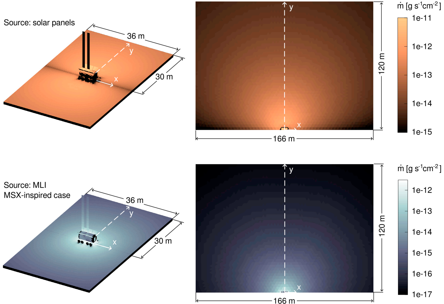
Figure 10. from S. Boccelli et al 2026 Planet. Sci. J. 7 doi:10.3847/PSJ/ae63c4 https://dx.doi.org/10.3847/PSJ/ae63c4 © 2026. The Author(s). Published by the American Astronomical Society.
