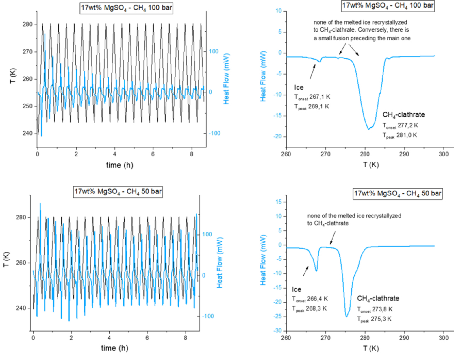
Figure A3. from Victoria Muñoz-Iglesias et al 2026 Planet. Sci. J. 7 doi:10.3847/PSJ/ae63c1 https://dx.doi.org/10.3847/PSJ/ae63c1 © 2026. The Author(s). Published by the American Astronomical Society.
