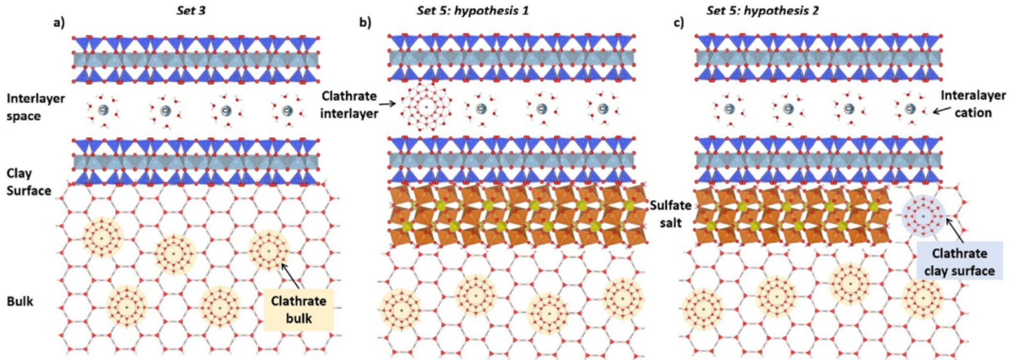
Figure 4. from Victoria Muñoz-Iglesias et al 2026 Planet. Sci. J. 7 doi:10.3847/PSJ/ae63c1 https://dx.doi.org/10.3847/PSJ/ae63c1 © 2026. The Author(s). Published by the American Astronomical Society.
