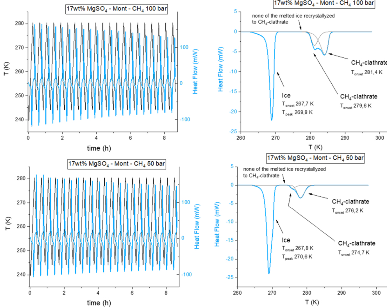
Figure A9. from Victoria Muñoz-Iglesias et al 2026 Planet. Sci. J. 7 doi:10.3847/PSJ/ae63c1 https://dx.doi.org/10.3847/PSJ/ae63c1 © 2026. The Author(s). Published by the American Astronomical Society.
