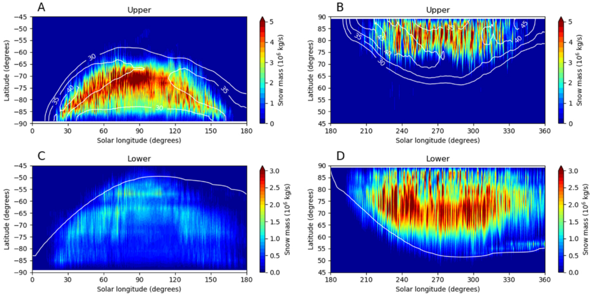
Figure 4. from Anthony D. Toigo et al 2026 Planet. Sci. J. 7 doi:10.3847/PSJ/ae63c0 https://dx.doi.org/10.3847/PSJ/ae63c0 © 2026. The Author(s). Published by the American Astronomical Society.
