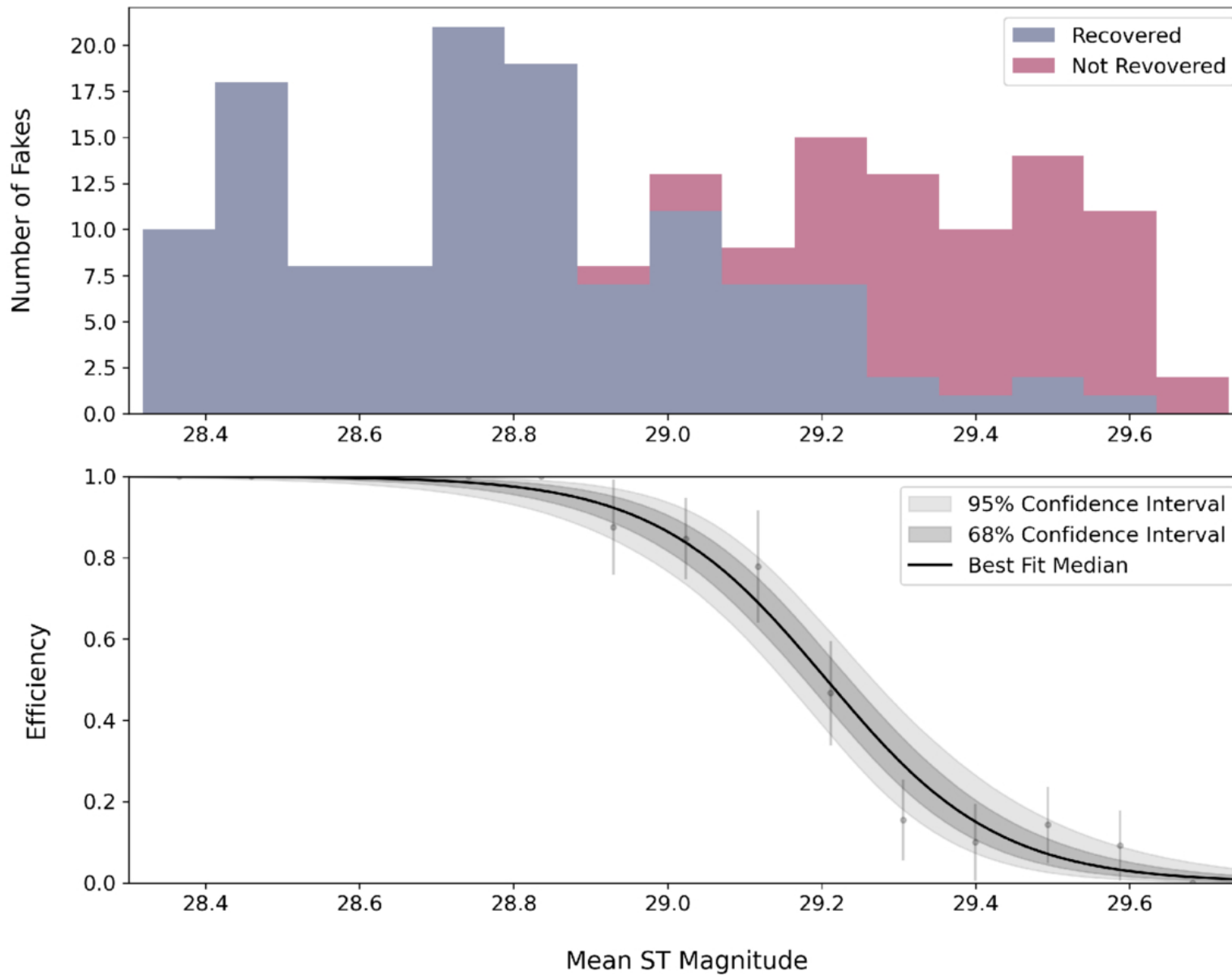
Figure 3. from Kevin J. Napier et al 2026 Planet. Sci. J. 7 doi:10.3847/PSJ/ae63b7 https://dx.doi.org/10.3847/PSJ/ae63b7 © 2026. The Author(s). Published by the American Astronomical Society.
