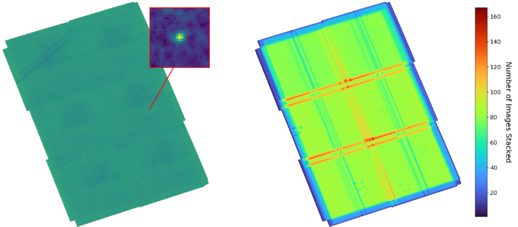
Figure 1. from Kevin J. Napier et al 2026 Planet. Sci. J. 7 doi:10.3847/PSJ/ae63b7 https://dx.doi.org/10.3847/PSJ/ae63b7 © 2026. The Author(s). Published by the American Astronomical Society.
