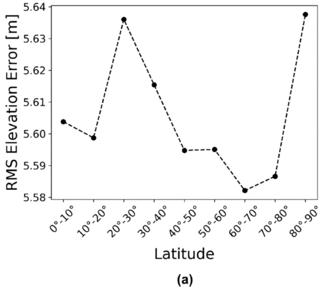
Figure 7. from Matthew Repasky et al 2026 Planet. Sci. J. 7 doi:10.3847/PSJ/ae6244 https://dx.doi.org/10.3847/PSJ/ae6244 © 2026. The Author(s). Published by the American Astronomical Society.
