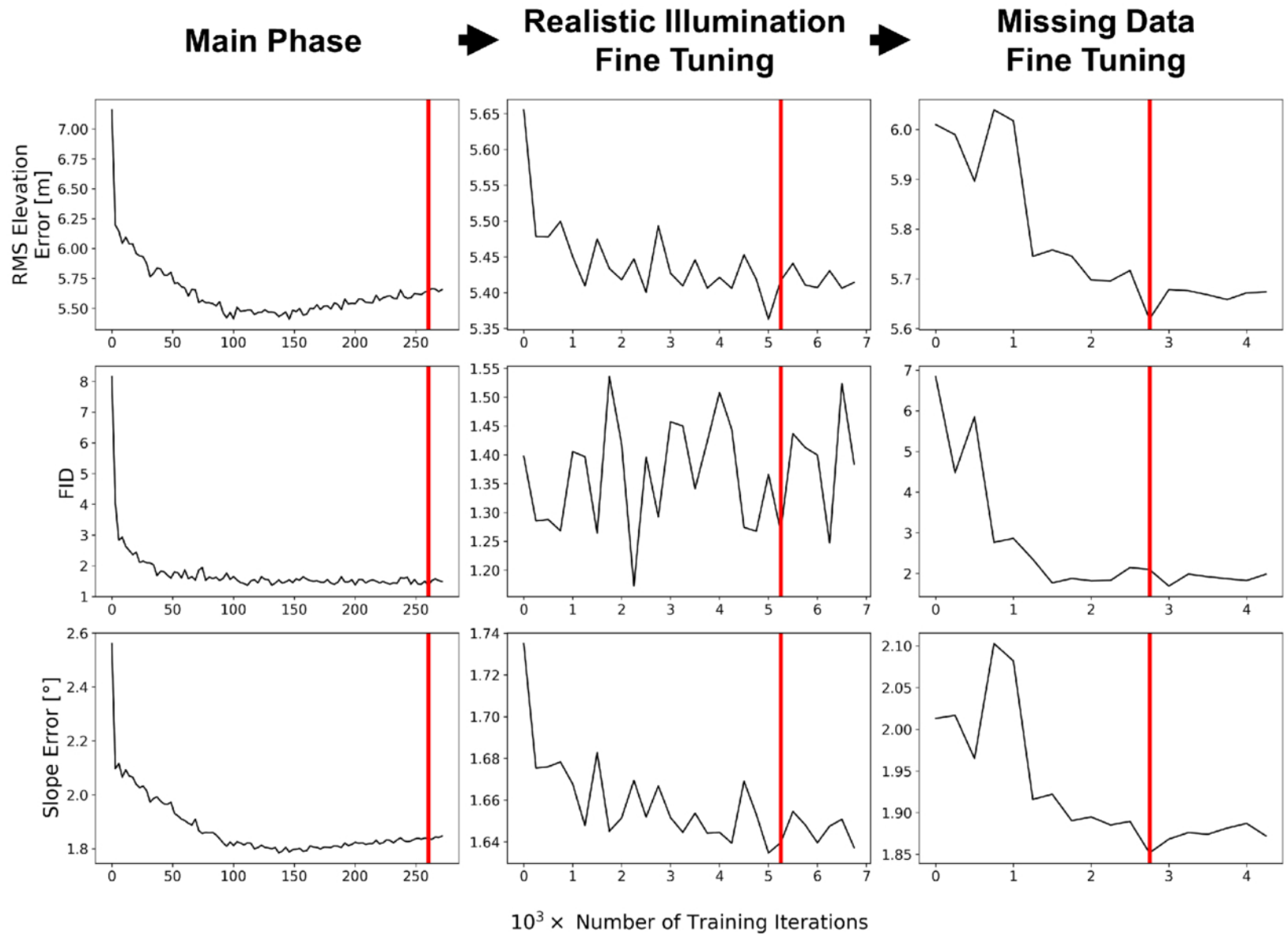
Figure 6. from Matthew Repasky et al 2026 Planet. Sci. J. 7 doi:10.3847/PSJ/ae6244 https://dx.doi.org/10.3847/PSJ/ae6244 © 2026. The Author(s). Published by the American Astronomical Society.
