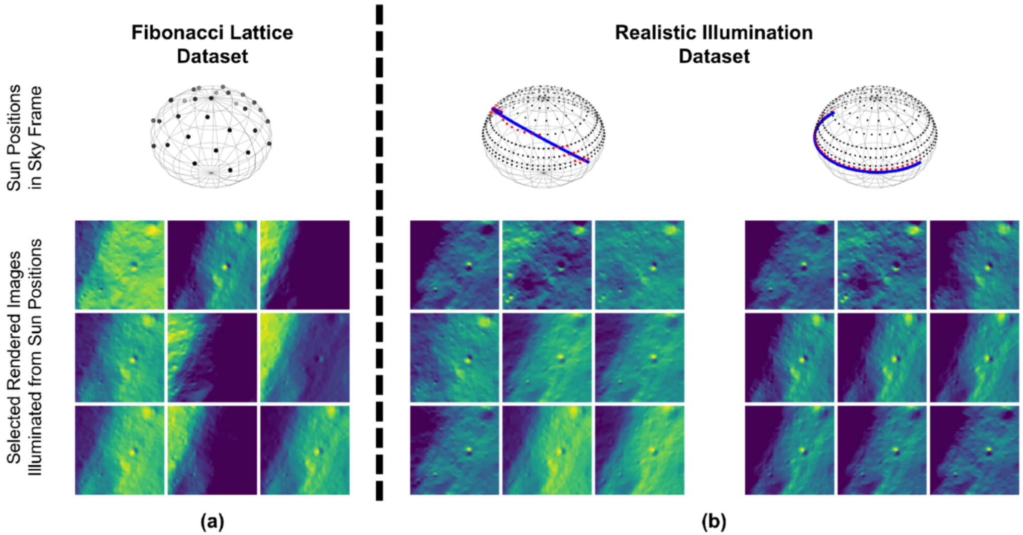
Figure 3. from Matthew Repasky et al 2026 Planet. Sci. J. 7 doi:10.3847/PSJ/ae6244 https://dx.doi.org/10.3847/PSJ/ae6244 © 2026. The Author(s). Published by the American Astronomical Society.
