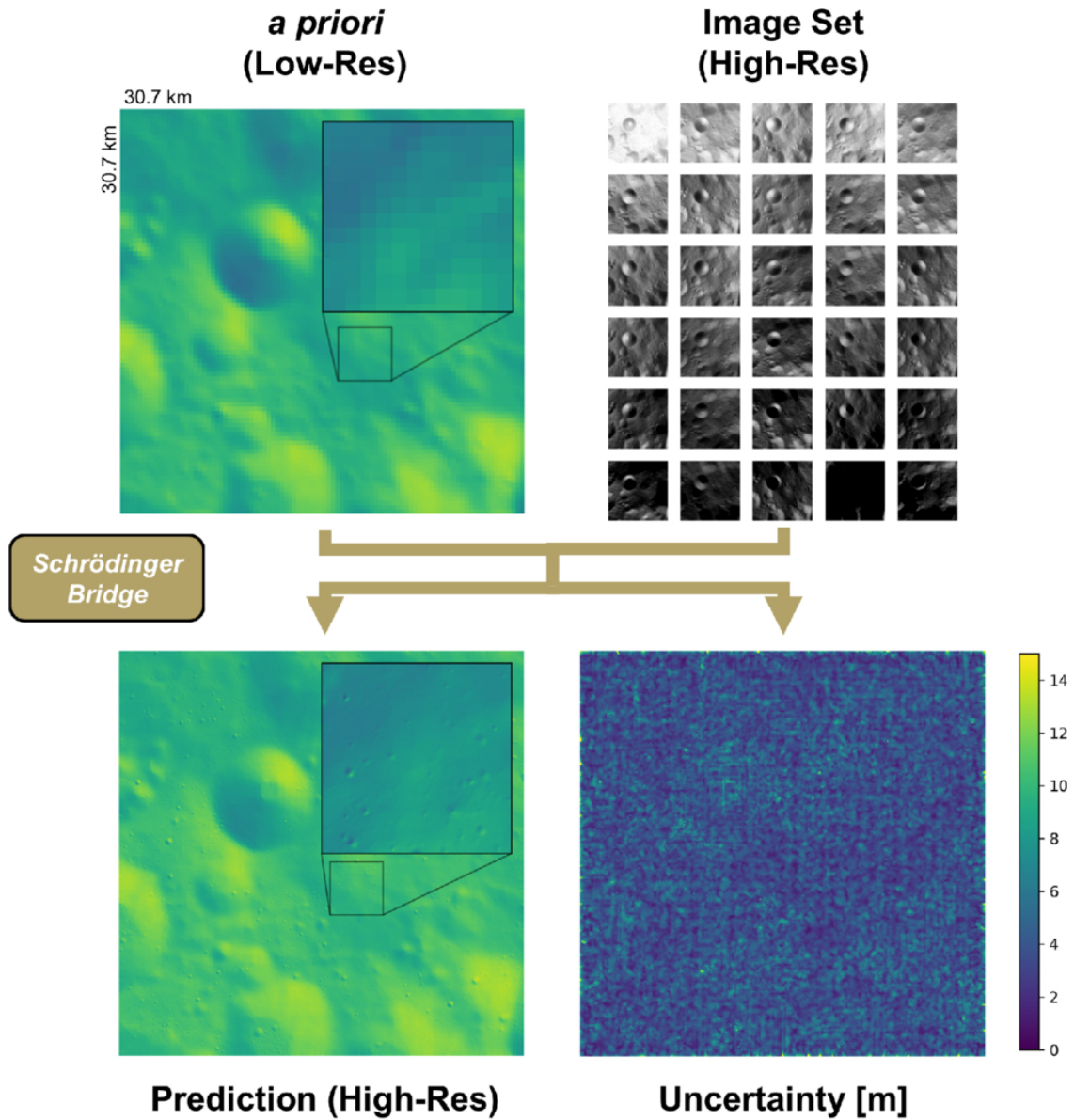
Figure 1. from Matthew Repasky et al 2026 Planet. Sci. J. 7 doi:10.3847/PSJ/ae6244 https://dx.doi.org/10.3847/PSJ/ae6244 © 2026. The Author(s). Published by the American Astronomical Society.
