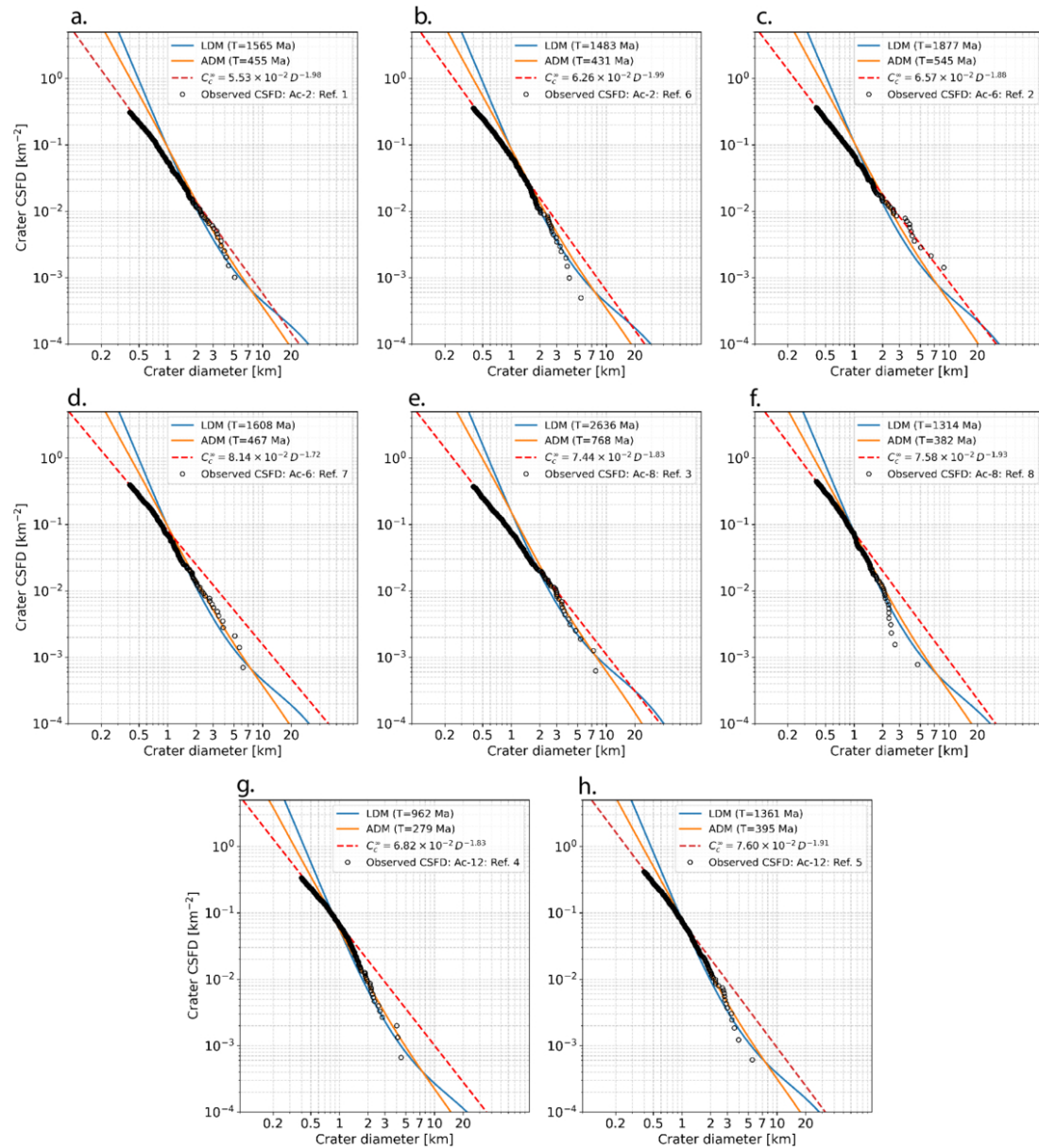
Figure 2. from Reem Vitale and Masatoshi Hirabayashi 2026 Planet. Sci. J. 7 doi:10.3847/PSJ/ae6241 https://dx.doi.org/10.3847/PSJ/ae6241 © 2026. The Author(s). Published by the American Astronomical Society.
