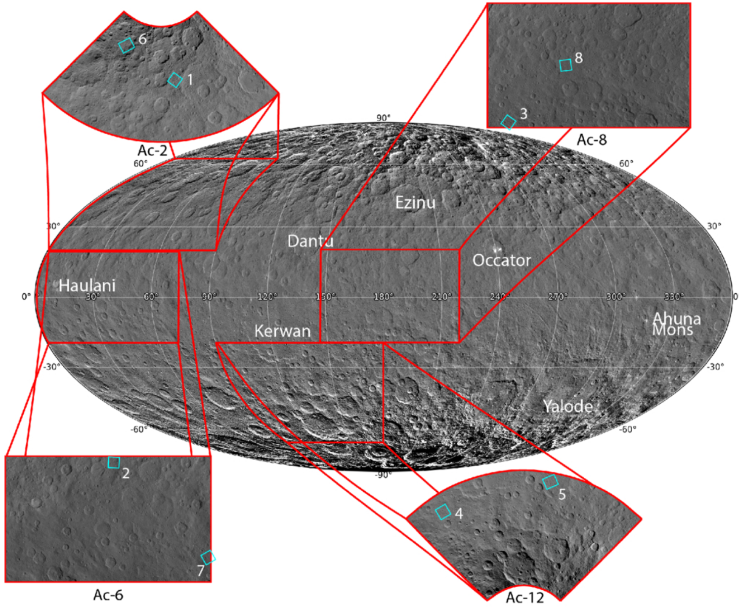
Figure 1. from Reem Vitale and Masatoshi Hirabayashi 2026 Planet. Sci. J. 7 doi:10.3847/PSJ/ae6241 https://dx.doi.org/10.3847/PSJ/ae6241 © 2026. The Author(s). Published by the American Astronomical Society.
