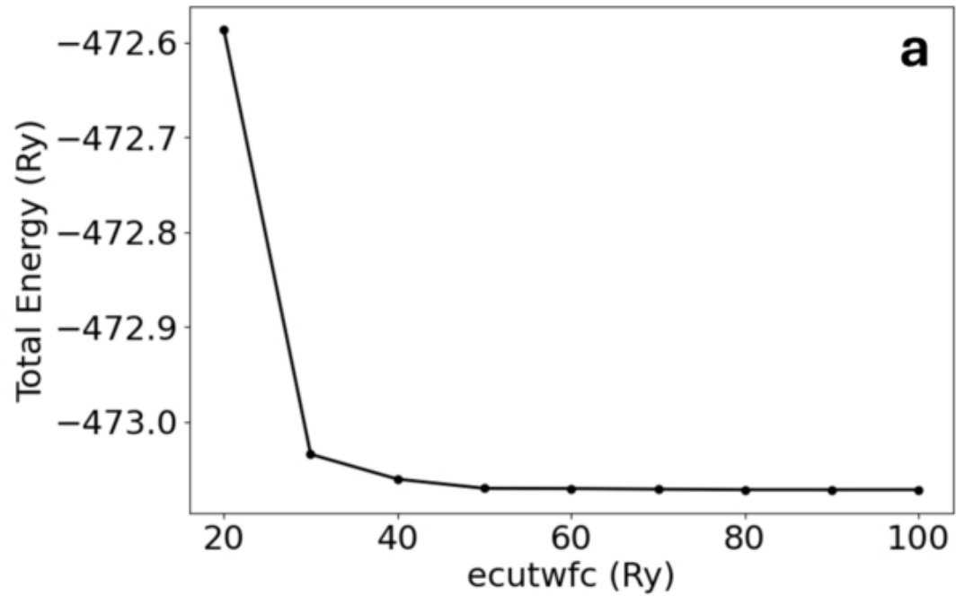
Figure A3. from Roshan S. Trivedi et al 2026 Planet. Sci. J. 7 doi:10.3847/PSJ/ae6074 https://dx.doi.org/10.3847/PSJ/ae6074 © 2026. The Author(s). Published by the American Astronomical Society.
