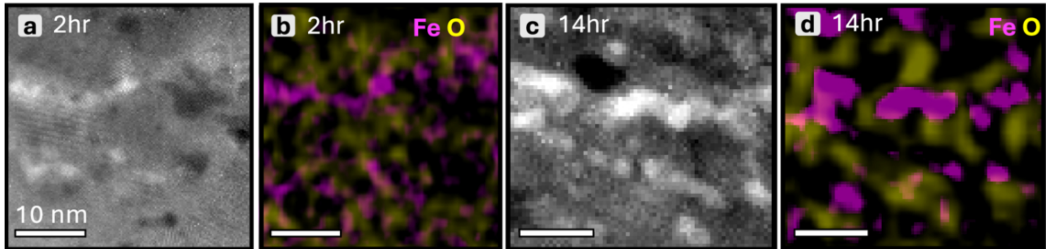
Figure A2. from Roshan S. Trivedi et al 2026 Planet. Sci. J. 7 doi:10.3847/PSJ/ae6074 https://dx.doi.org/10.3847/PSJ/ae6074 © 2026. The Author(s). Published by the American Astronomical Society.
