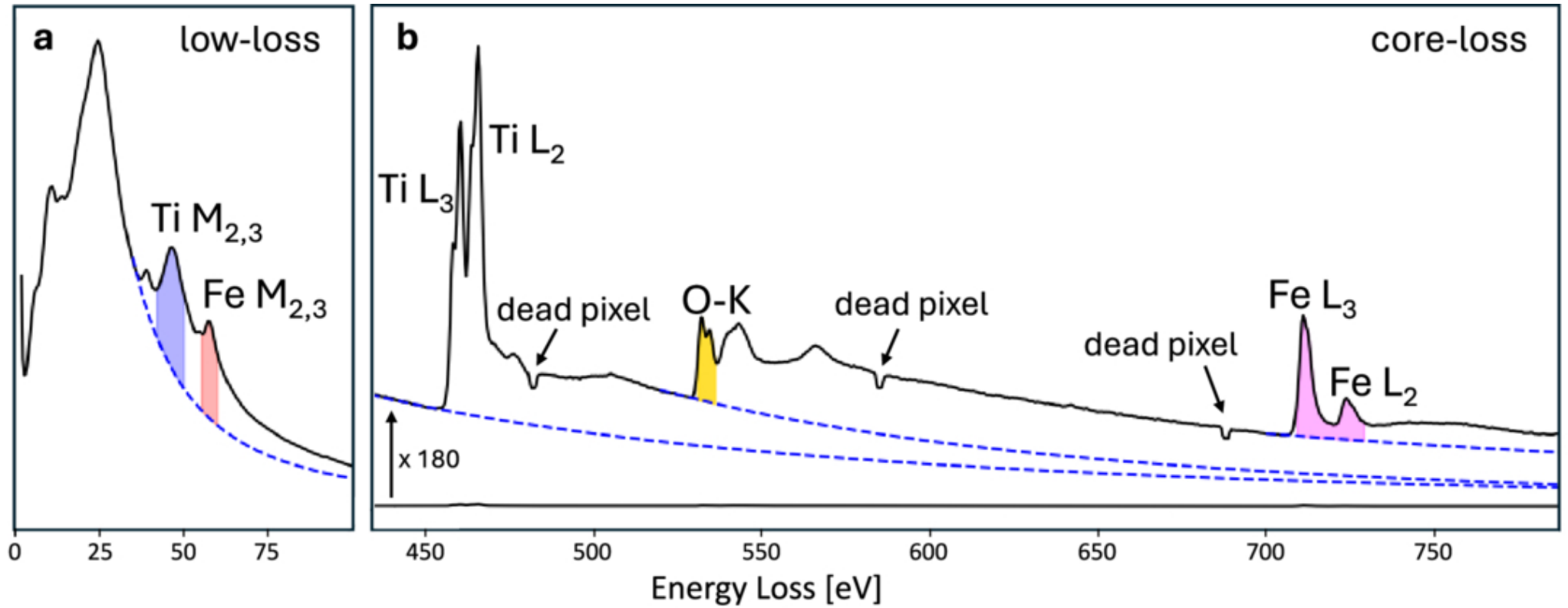
Figure A1. from Roshan S. Trivedi et al 2026 Planet. Sci. J. 7 doi:10.3847/PSJ/ae6074 https://dx.doi.org/10.3847/PSJ/ae6074 © 2026. The Author(s). Published by the American Astronomical Society.
