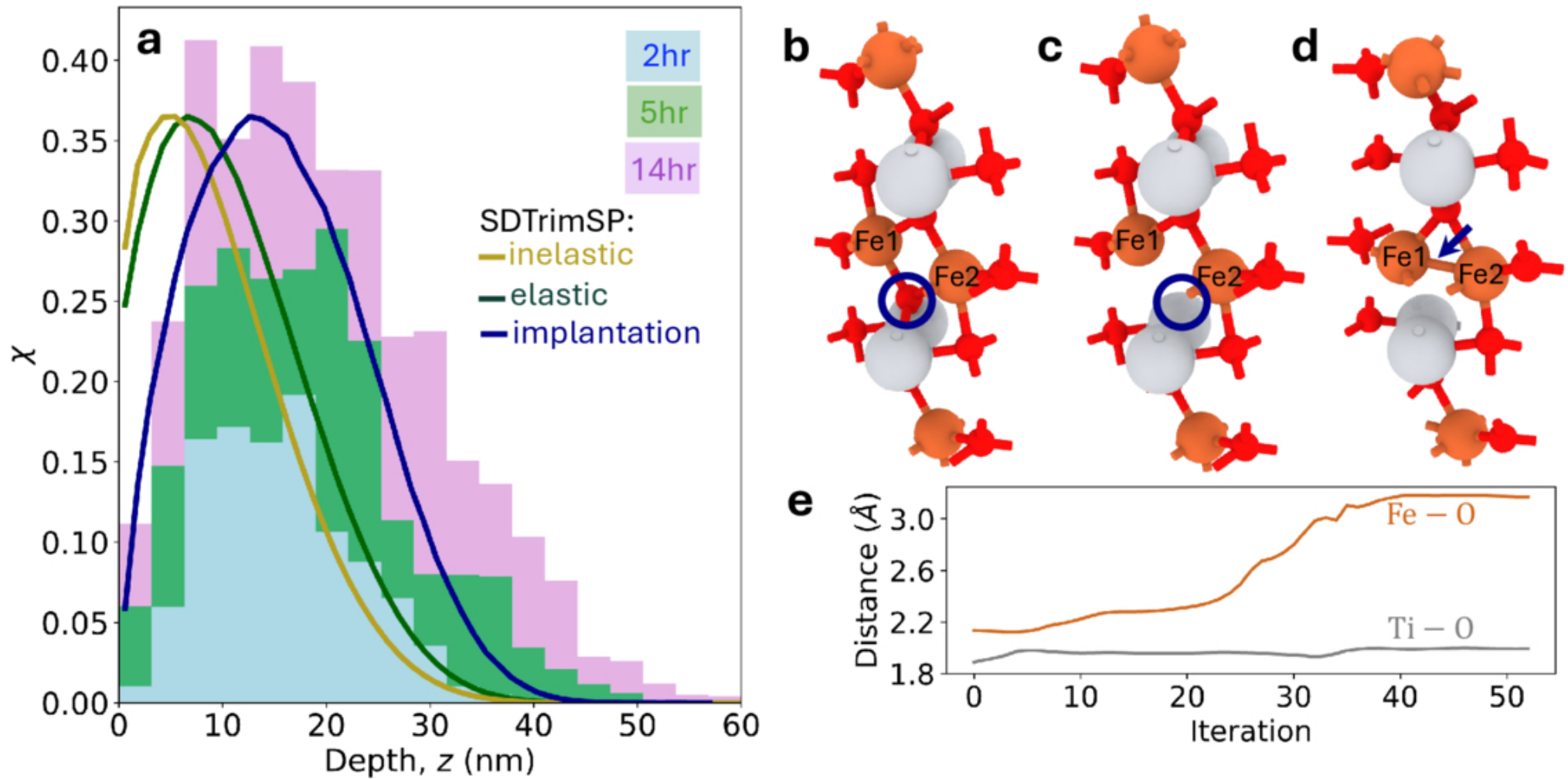
Figure 6. from Roshan S. Trivedi et al 2026 Planet. Sci. J. 7 doi:10.3847/PSJ/ae6074 https://dx.doi.org/10.3847/PSJ/ae6074 © 2026. The Author(s). Published by the American Astronomical Society.
