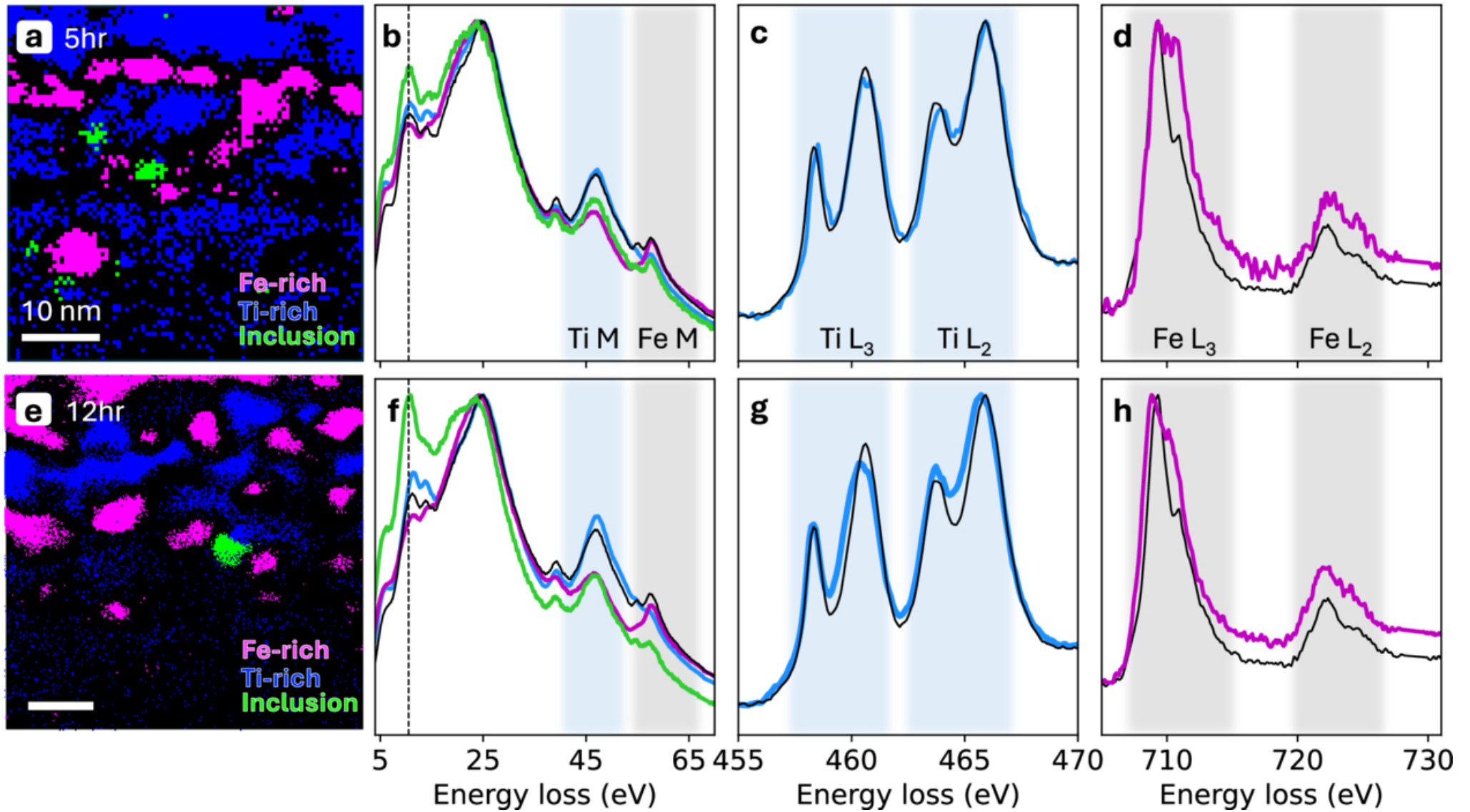
Figure 4. from Roshan S. Trivedi et al 2026 Planet. Sci. J. 7 doi:10.3847/PSJ/ae6074 https://dx.doi.org/10.3847/PSJ/ae6074 © 2026. The Author(s). Published by the American Astronomical Society.
