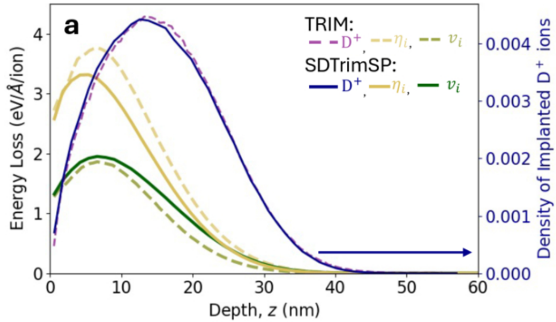
Figure A8. from Roshan S. Trivedi et al 2026 Planet. Sci. J. 7 doi:10.3847/PSJ/ae6074 https://dx.doi.org/10.3847/PSJ/ae6074 © 2026. The Author(s). Published by the American Astronomical Society.
