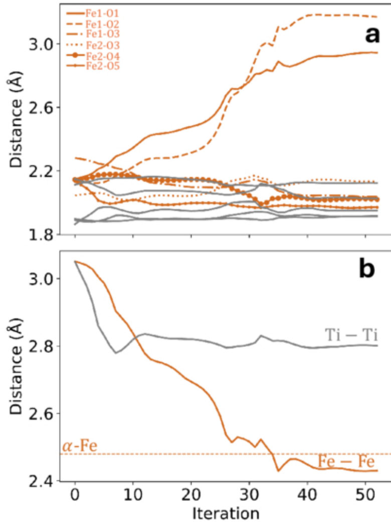
Figure A7. from Roshan S. Trivedi et al 2026 Planet. Sci. J. 7 doi:10.3847/PSJ/ae6074 https://dx.doi.org/10.3847/PSJ/ae6074 © 2026. The Author(s). Published by the American Astronomical Society.
