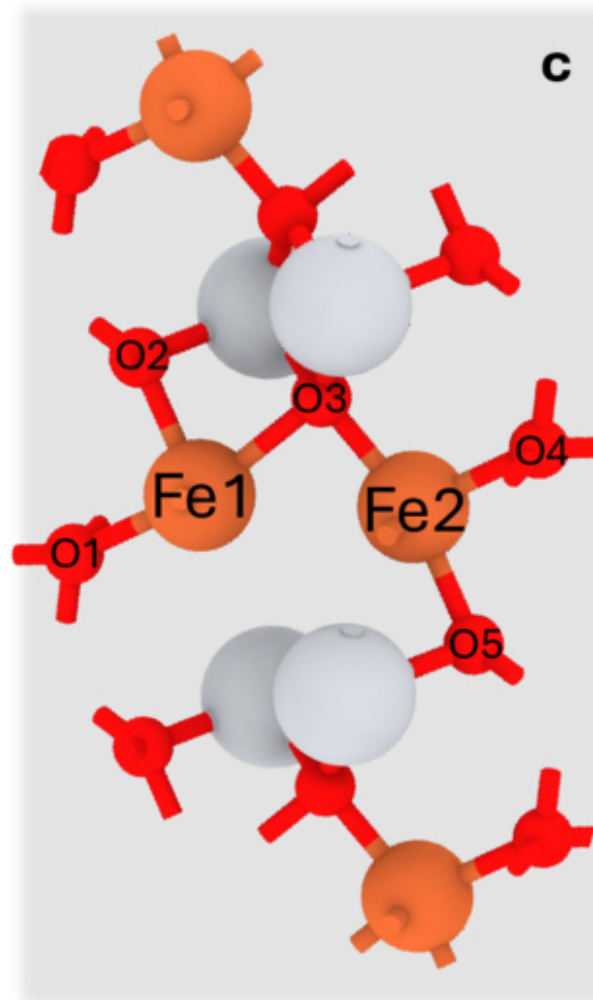
Figure A7. from Roshan S. Trivedi et al 2026 Planet. Sci. J. 7 doi:10.3847/PSJ/ae6074 https://dx.doi.org/10.3847/PSJ/ae6074 © 2026. The Author(s). Published by the American Astronomical Society.
