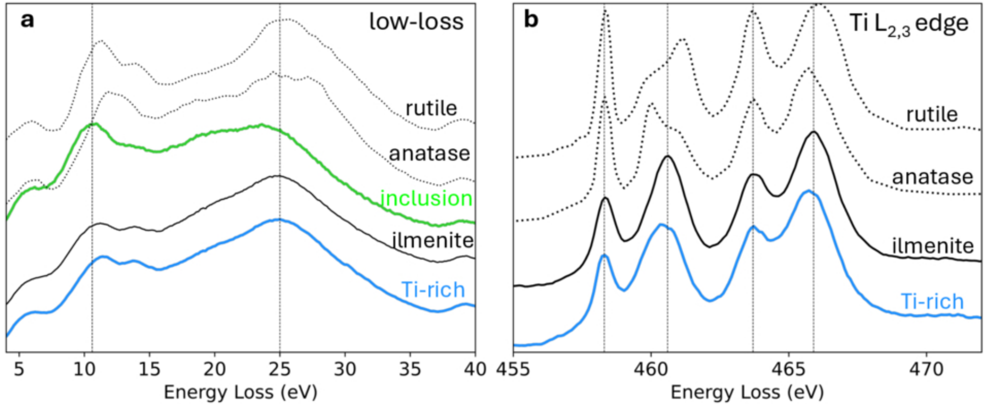
Figure A6. from Roshan S. Trivedi et al 2026 Planet. Sci. J. 7 doi:10.3847/PSJ/ae6074 https://dx.doi.org/10.3847/PSJ/ae6074 © 2026. The Author(s). Published by the American Astronomical Society.
