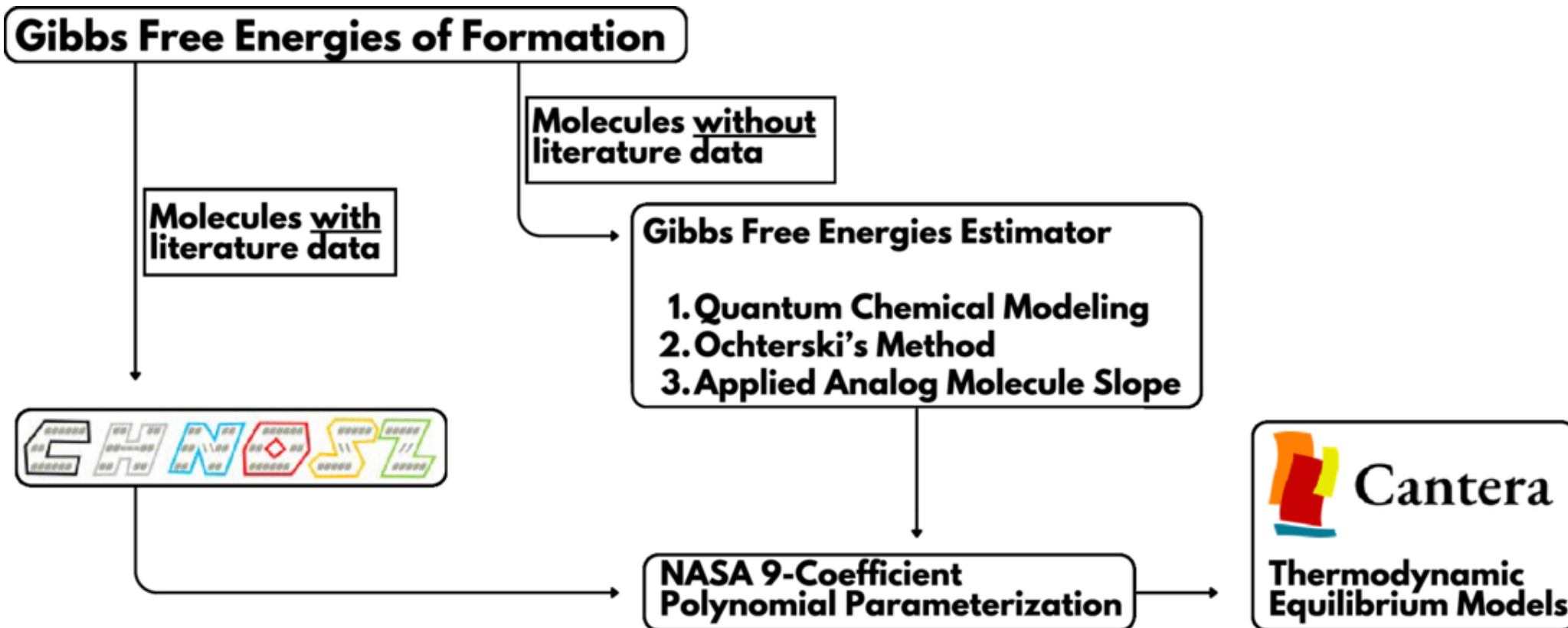
Figure 1. from Ishaan Madan and Ben K. D. Pearce 2026 Planet. Sci. J. 7 doi:10.3847/PSJ/ae5f91 https://dx.doi.org/10.3847/PSJ/ae5f91 © 2026. The Author(s). Published by the American Astronomical Society.
