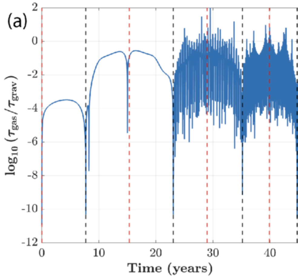
Figure 6. from Ketan Kamat et al 2026 Planet. Sci. J. 7 doi:10.3847/PSJ/ae5f8e https://dx.doi.org/10.3847/PSJ/ae5f8e © 2026. The Author(s). Published by the American Astronomical Society.
