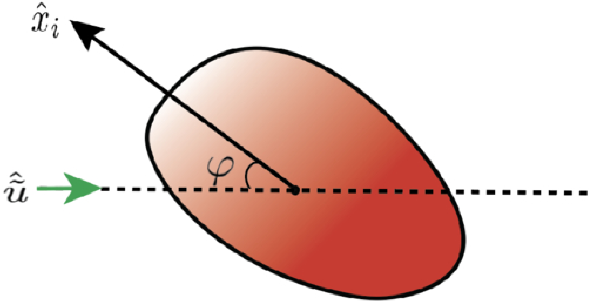
Figure 5. from Ketan Kamat et al 2026 Planet. Sci. J. 7 doi:10.3847/PSJ/ae5f8e https://dx.doi.org/10.3847/PSJ/ae5f8e © 2026. The Author(s). Published by the American Astronomical Society.
