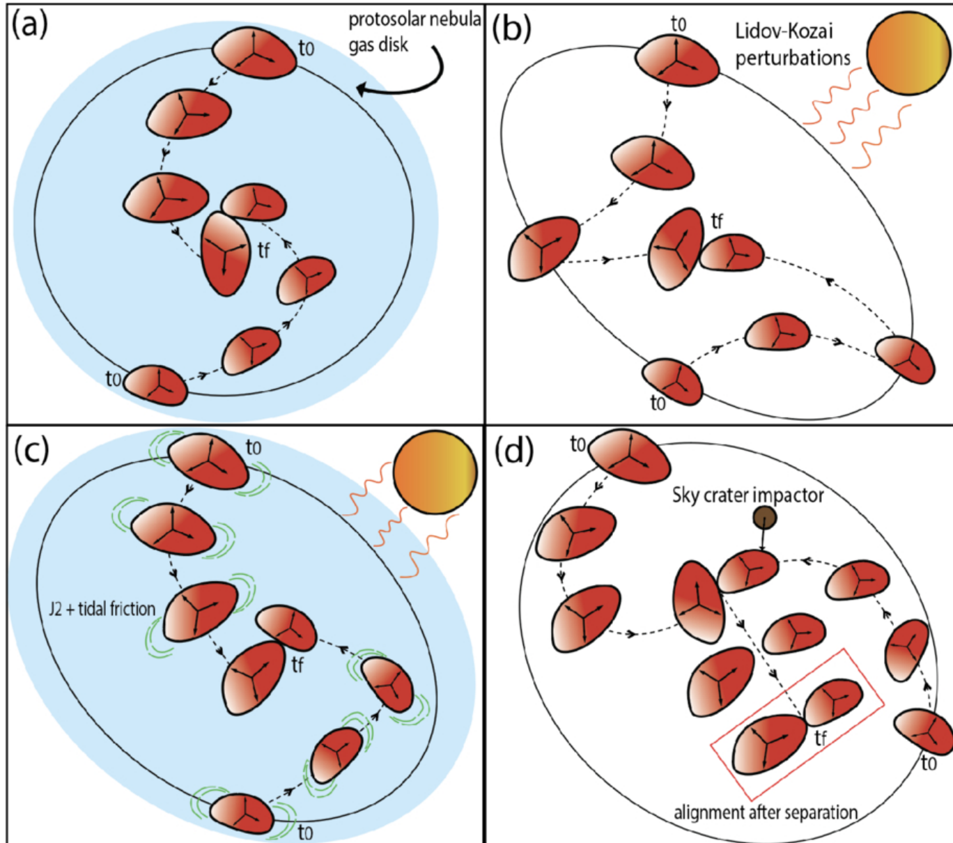
Figure 11. from Ketan Kamat et al 2026 Planet. Sci. J. 7 doi:10.3847/PSJ/ae5f8e https://dx.doi.org/10.3847/PSJ/ae5f8e © 2026. The Author(s). Published by the American Astronomical Society.
