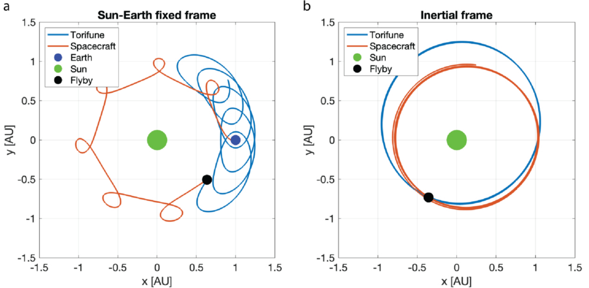
Figure 2. from Masatoshi Hirabayashi et al 2026 Planet. Sci. J. 7 doi:10.3847/PSJ/ae5f79 https://dx.doi.org/10.3847/PSJ/ae5f79 © 2026. The Author(s). Published by the American Astronomical Society.
