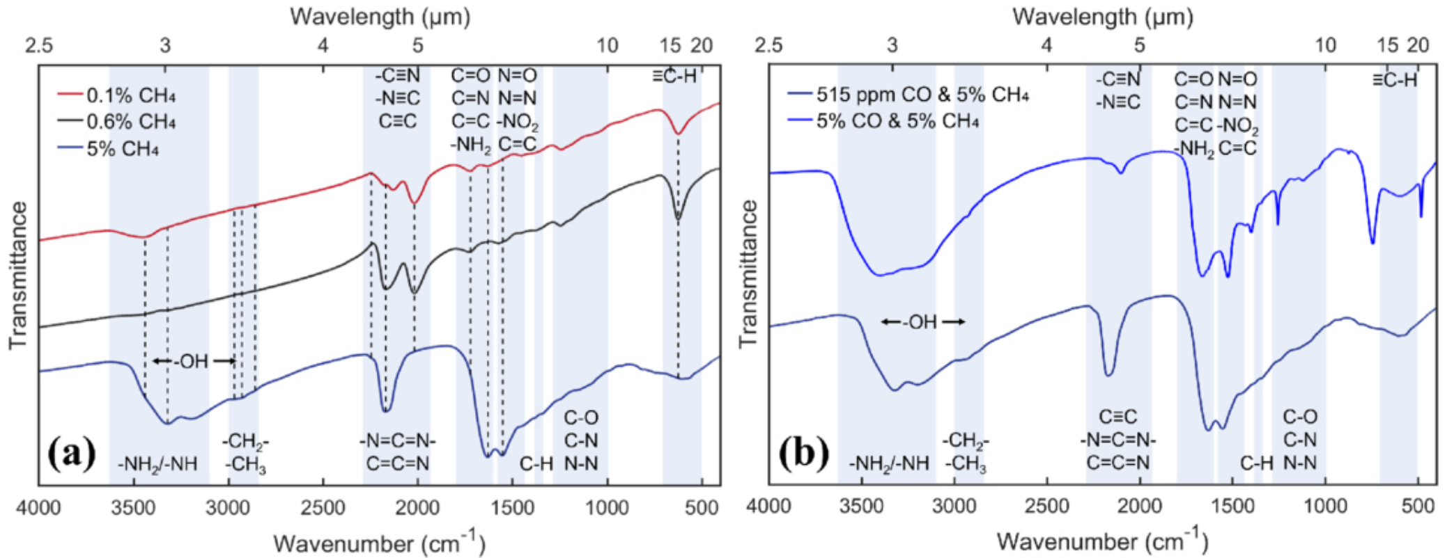
Figure 3. from Zhengbo Yang et al 2026 Planet. Sci. J. 7 doi:10.3847/PSJ/ae5e70 https://dx.doi.org/10.3847/PSJ/ae5e70 © 2026. The Author(s). Published by the American Astronomical Society.
