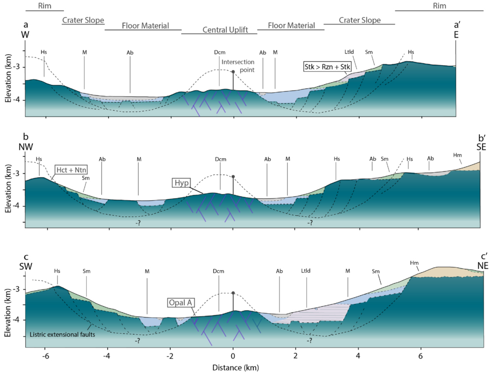
Figure 8. from M. C. Rojas et al 2026 Planet. Sci. J. 7 doi:10.3847/PSJ/ae5dcb https://dx.doi.org/10.3847/PSJ/ae5dcb © 2026. The Author(s). Published by the American Astronomical Society.
