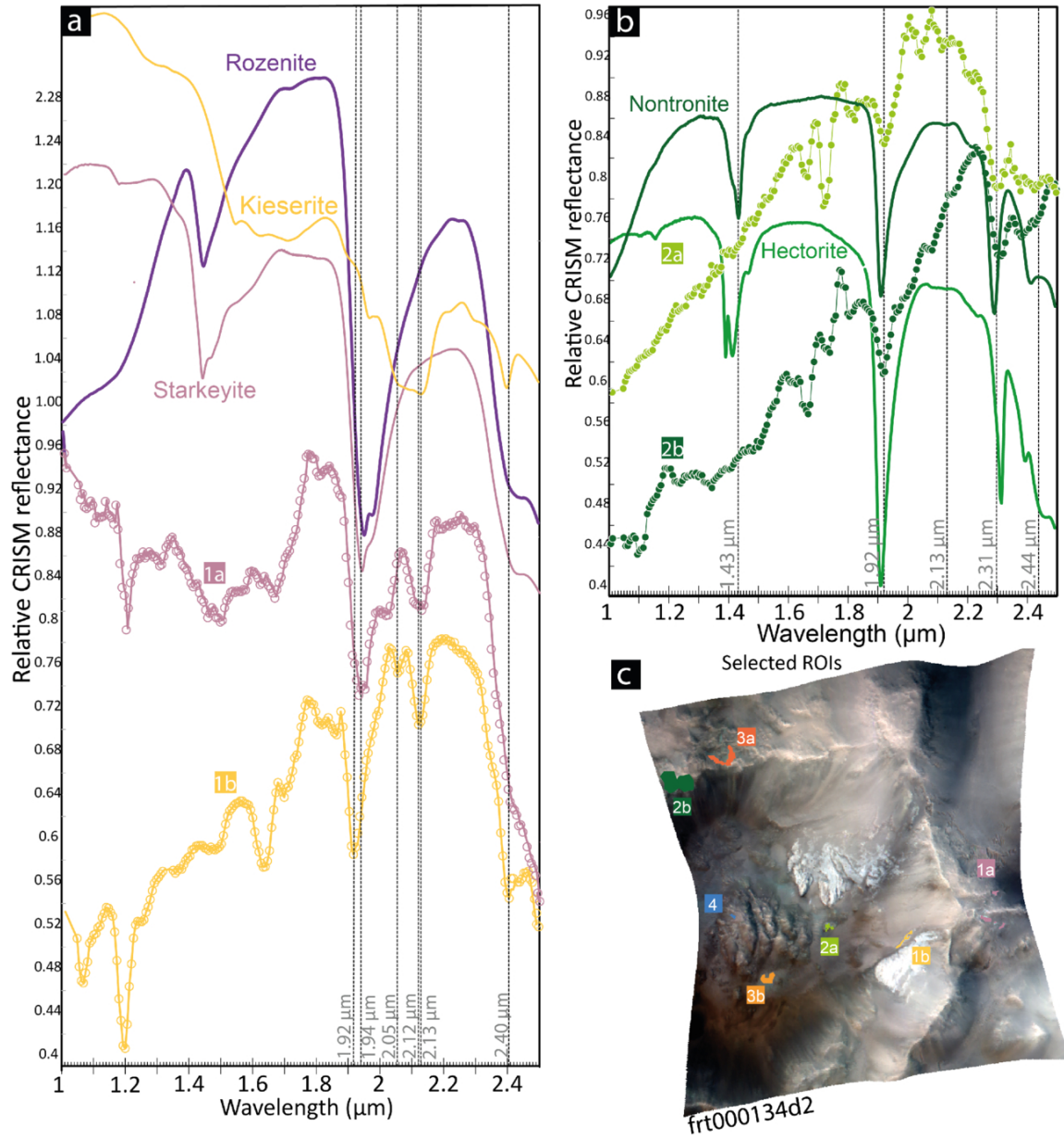
Figure 5. from M. C. Rojas et al 2026 Planet. Sci. J. 7 doi:10.3847/PSJ/ae5dcb https://dx.doi.org/10.3847/PSJ/ae5dcb © 2026. The Author(s). Published by the American Astronomical Society.
