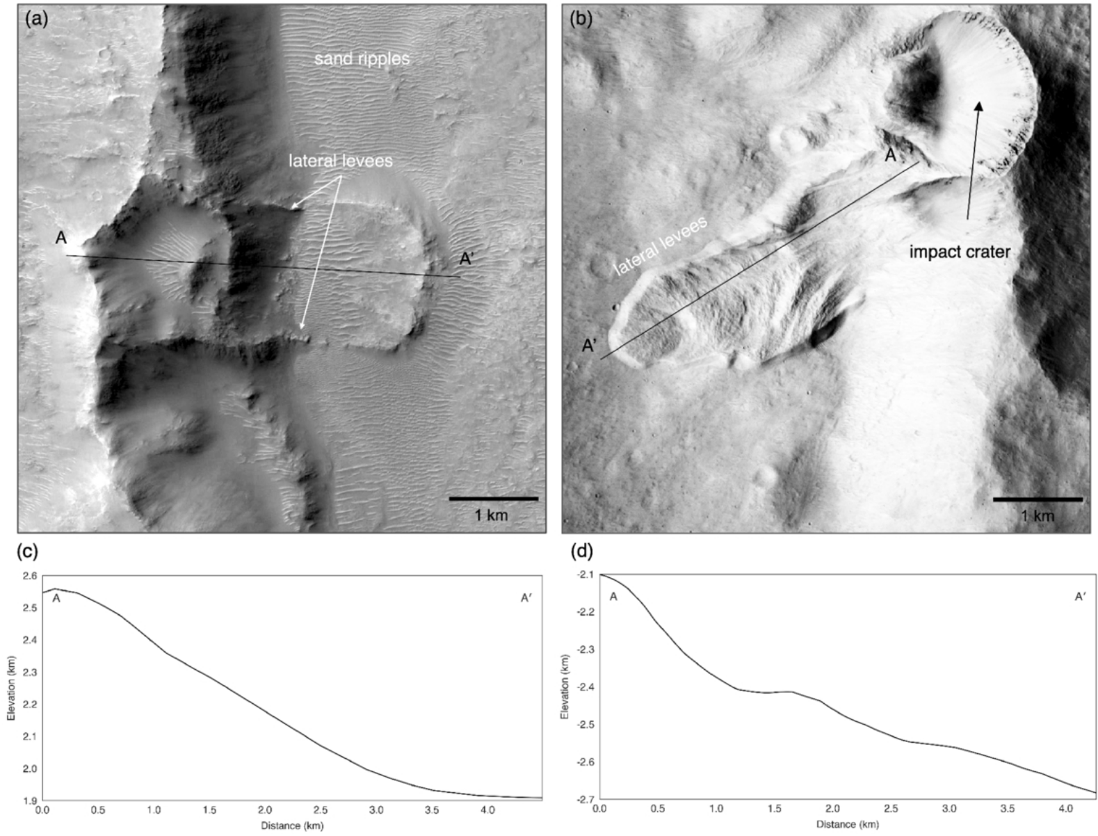
Figure 8. from Yunwan Tao et al 2026 Planet. Sci. J. 7 doi:10.3847/PSJ/ae5dc7 https://dx.doi.org/10.3847/PSJ/ae5dc7 © 2026. The Author(s). Published by the American Astronomical Society.
