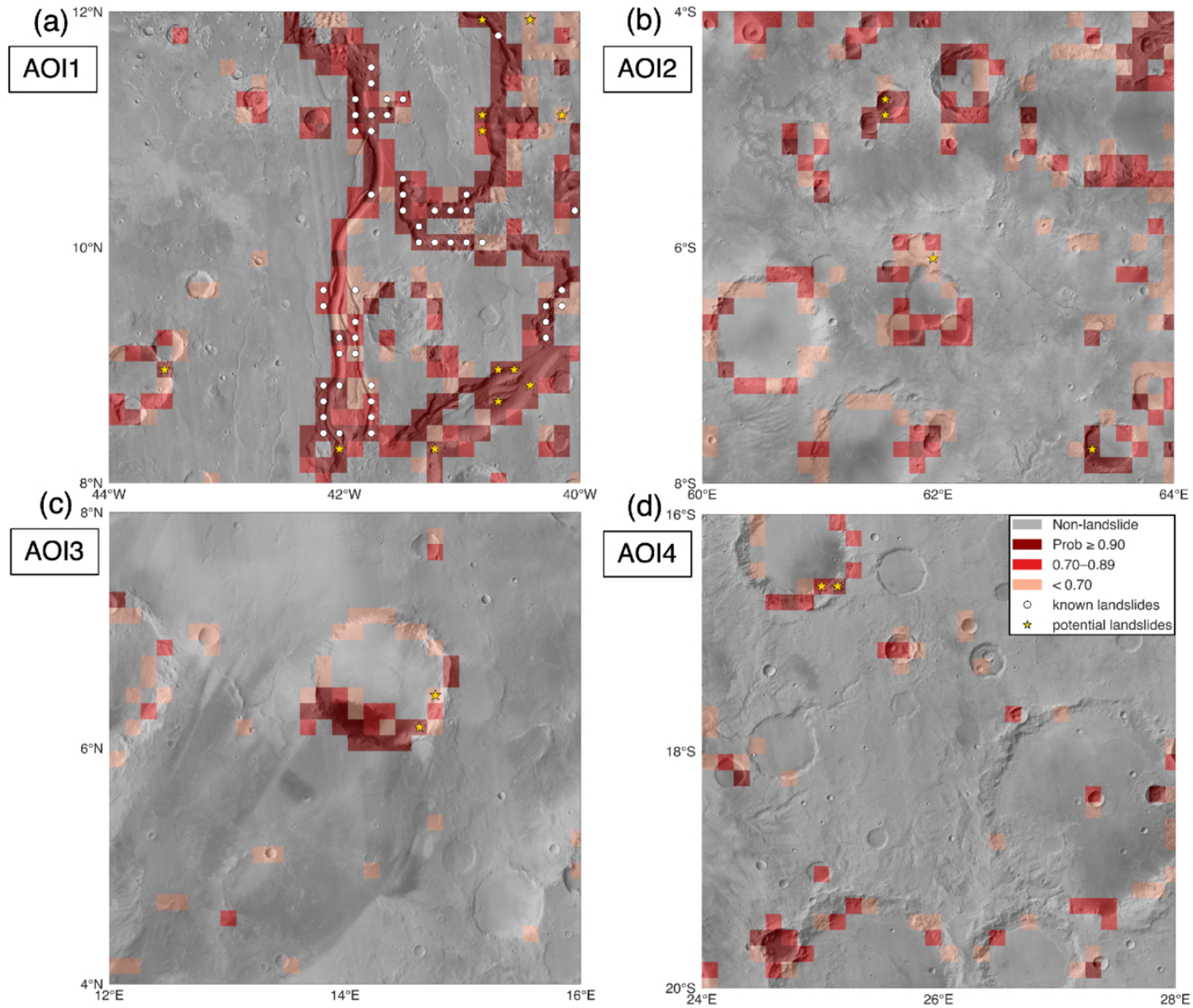
Figure 6. from Yunwan Tao et al 2026 Planet. Sci. J. 7 doi:10.3847/PSJ/ae5dc7 https://dx.doi.org/10.3847/PSJ/ae5dc7 © 2026. The Author(s). Published by the American Astronomical Society.
