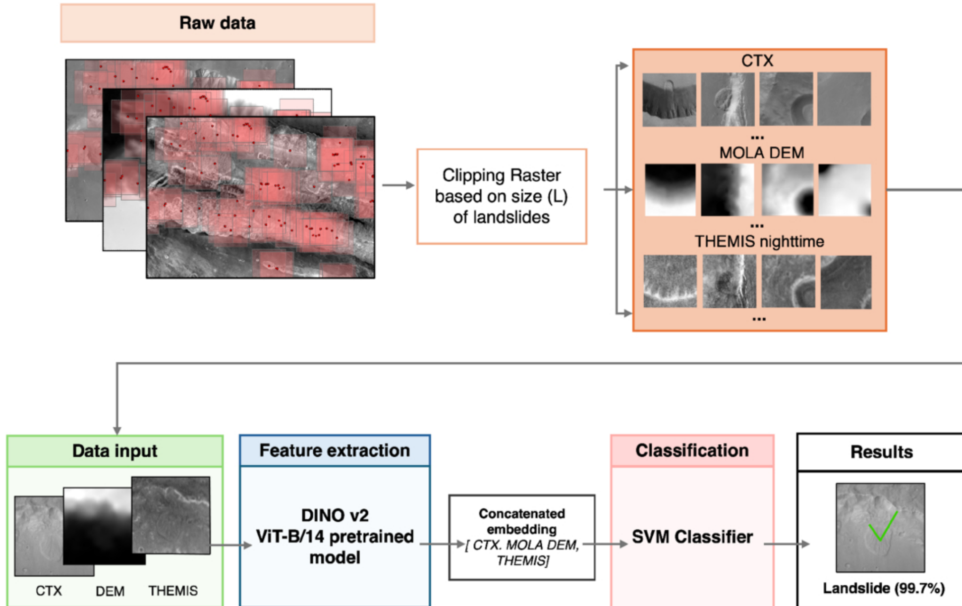
Figure 4. from Yunwan Tao et al 2026 Planet. Sci. J. 7 doi:10.3847/PSJ/ae5dc7 https://dx.doi.org/10.3847/PSJ/ae5dc7 © 2026. The Author(s). Published by the American Astronomical Society.
