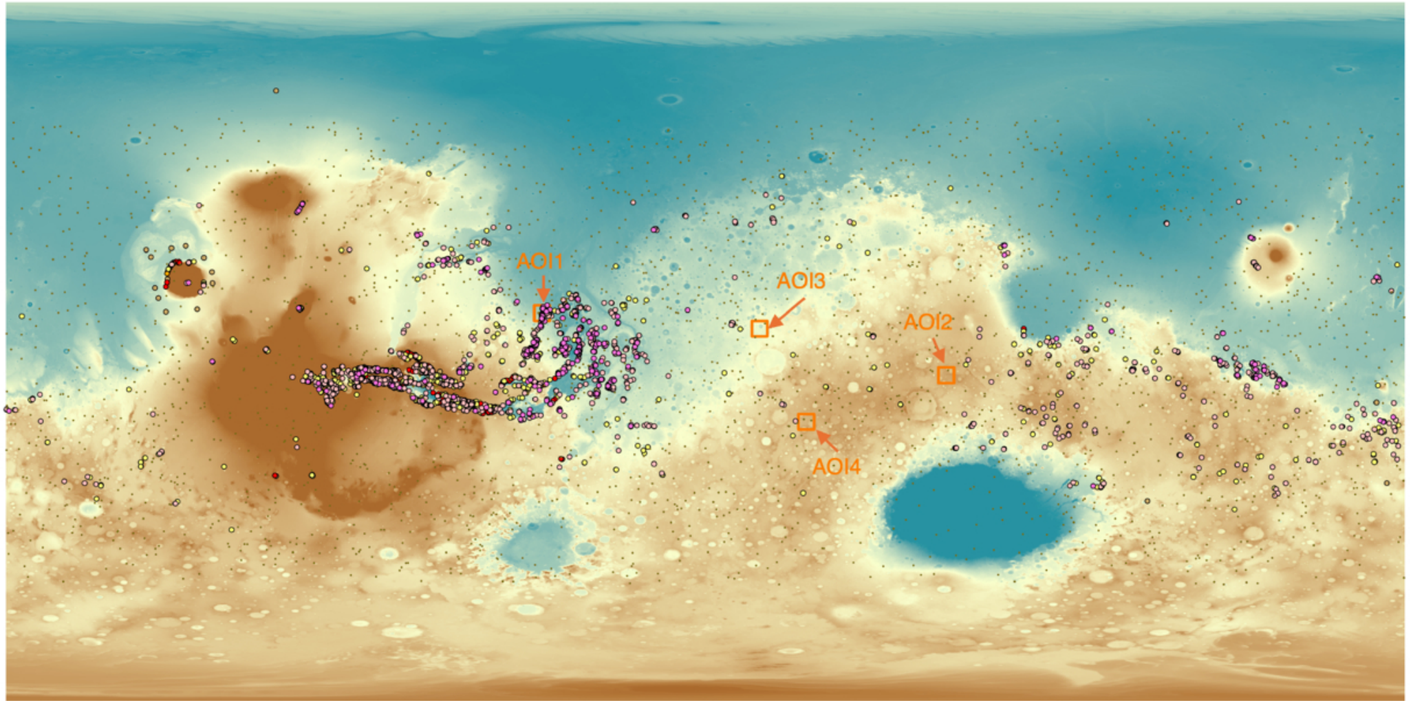
Figure 1. from Yunwan Tao et al 2026 Planet. Sci. J. 7 doi:10.3847/PSJ/ae5dc7 https://dx.doi.org/10.3847/PSJ/ae5dc7 © 2026. The Author(s). Published by the American Astronomical Society.
