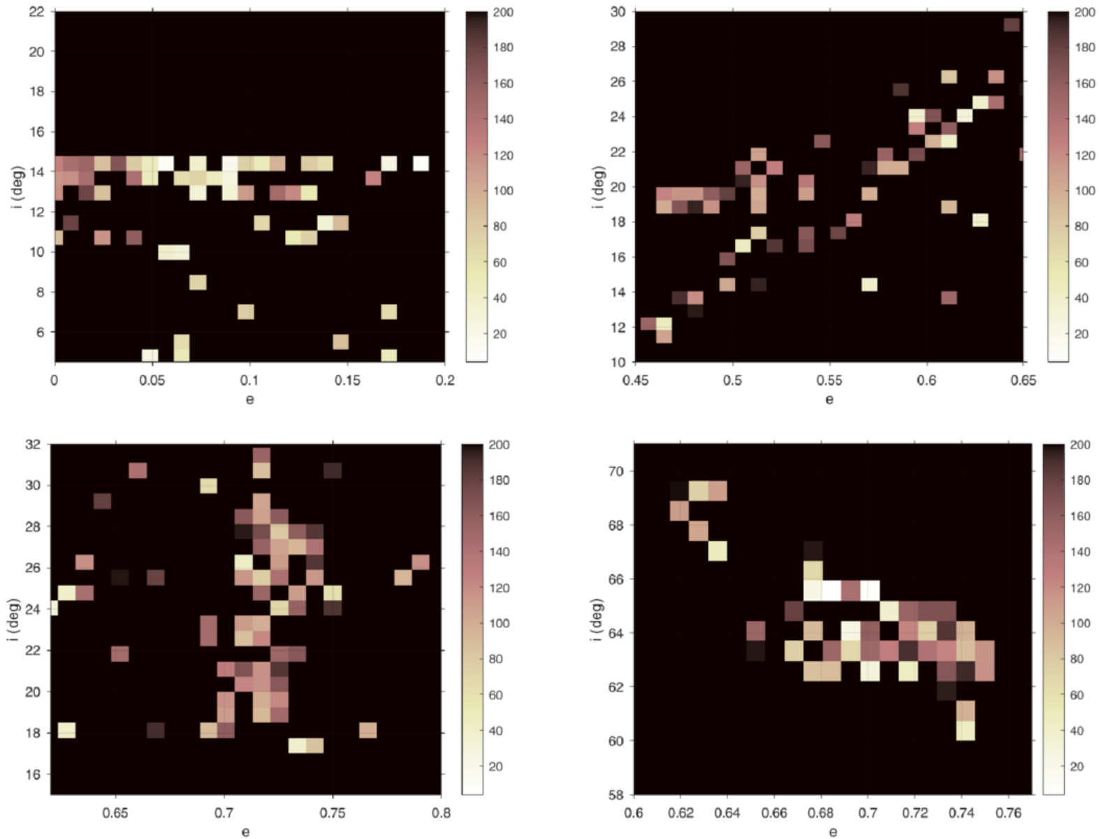
Figure 6. from Giulia Schettino and Alessandro Rossi 2026 Planet. Sci. J. 7 doi:10.3847/PSJ/ae5dc3 https://dx.doi.org/10.3847/PSJ/ae5dc3 © 2026. The Author(s). Published by the American Astronomical Society.
