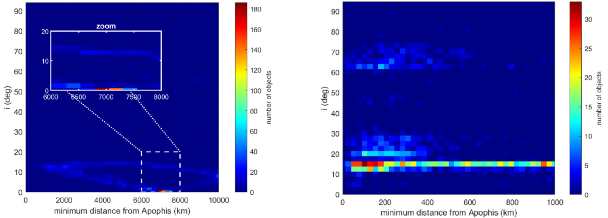
Figure 2. from Giulia Schettino and Alessandro Rossi 2026 Planet. Sci. J. 7 doi:10.3847/PSJ/ae5dc3 https://dx.doi.org/10.3847/PSJ/ae5dc3 © 2026. The Author(s). Published by the American Astronomical Society.
