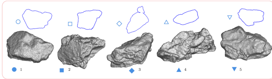
Figure 9. from Alexia Duchêne et al 2026 Planet. Sci. J. 7 doi:10.3847/PSJ/ae5d37 https://dx.doi.org/10.3847/PSJ/ae5d37 © 2026. The Author(s). Published by the American Astronomical Society.
