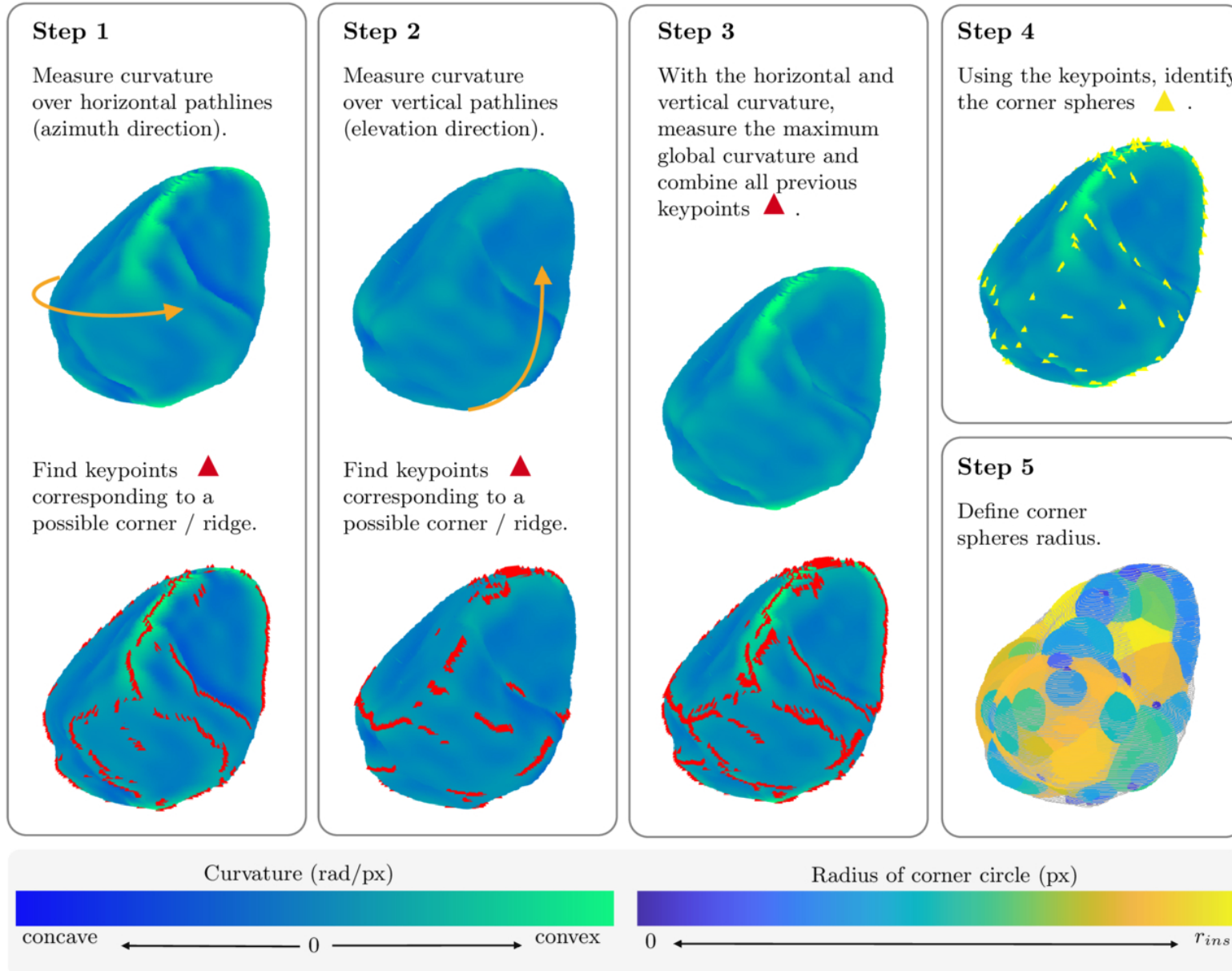
Figure 5. from Alexia Duchêne et al 2026 Planet. Sci. J. 7 doi:10.3847/PSJ/ae5d37 https://dx.doi.org/10.3847/PSJ/ae5d37 © 2026. The Author(s). Published by the American Astronomical Society.
