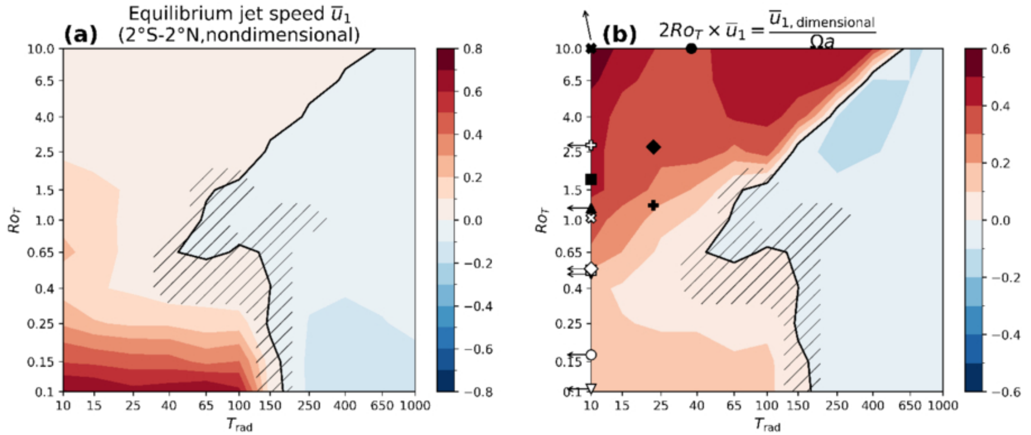
Figure 5. from Quentin Nicolas and Geoffrey K. Vallis 2026 Planet. Sci. J. 7 doi:10.3847/PSJ/ae5c96 https://dx.doi.org/10.3847/PSJ/ae5c96 © 2026. The Author(s). Published by the American Astronomical Society.
