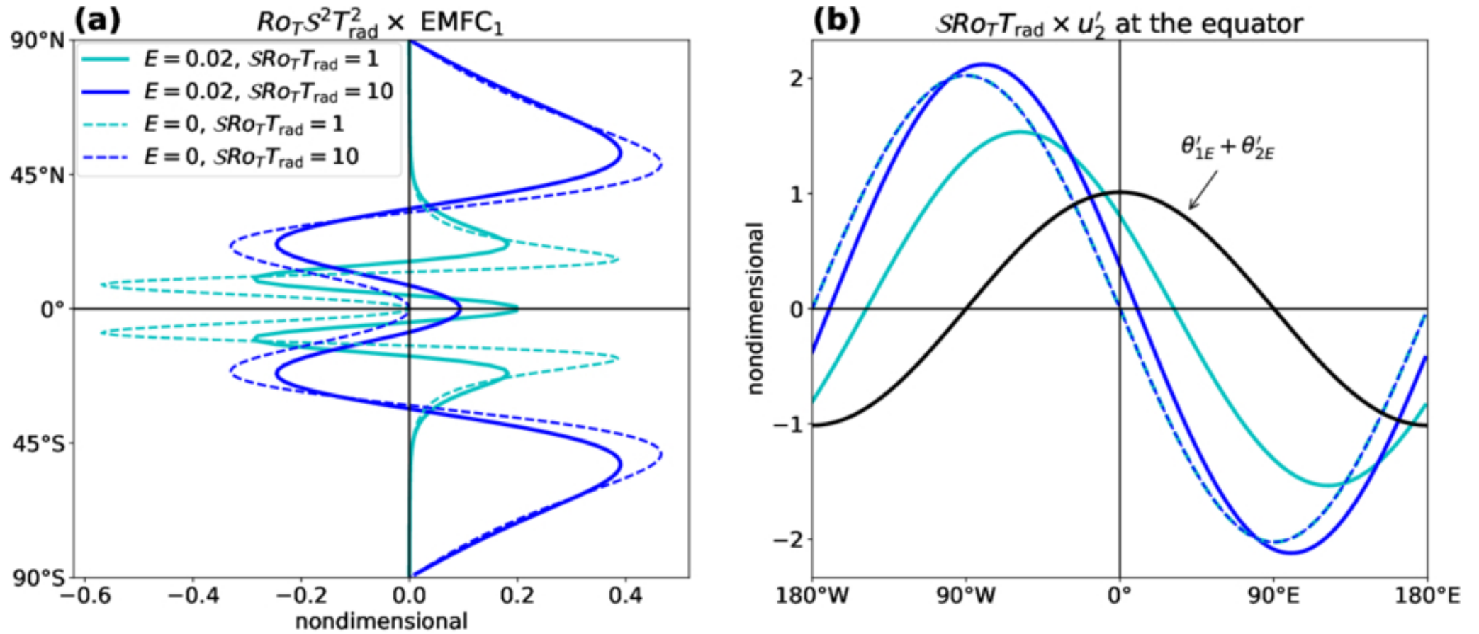
Figure 3. from Quentin Nicolas and Geoffrey K. Vallis 2026 Planet. Sci. J. 7 doi:10.3847/PSJ/ae5c96 https://dx.doi.org/10.3847/PSJ/ae5c96 © 2026. The Author(s). Published by the American Astronomical Society.
