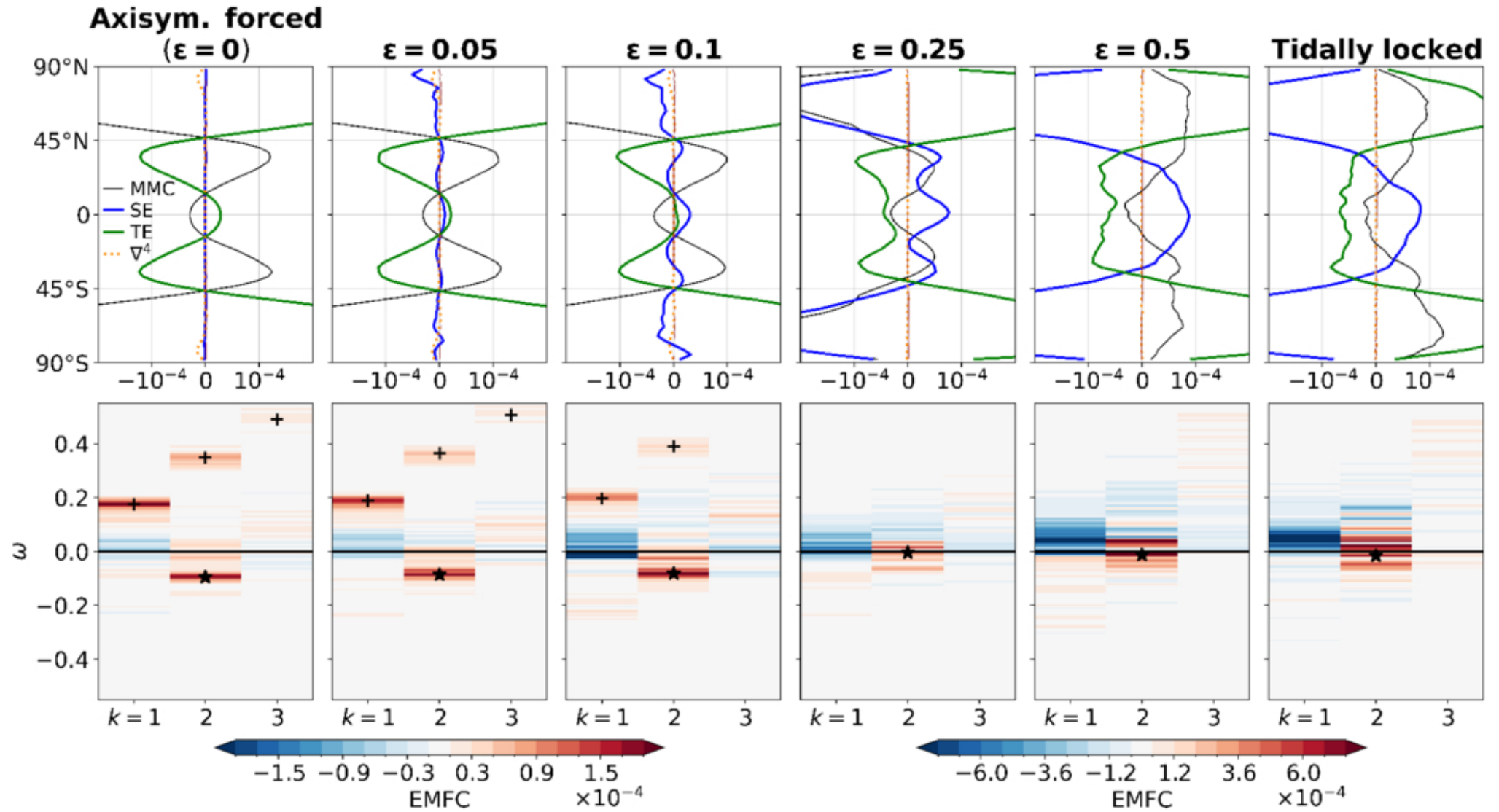
Figure 14. from Quentin Nicolas and Geoffrey K. Vallis 2026 Planet. Sci. J. 7 doi:10.3847/PSJ/ae5c96 https://dx.doi.org/10.3847/PSJ/ae5c96 © 2026. The Author(s). Published by the American Astronomical Society.
