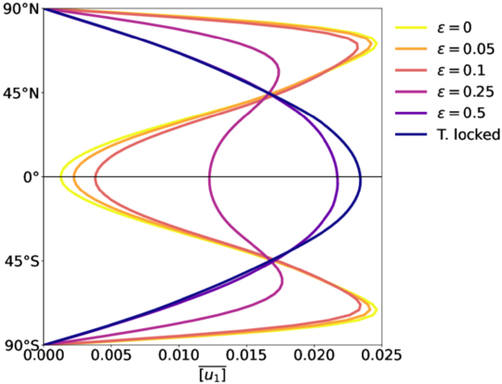
Figure 13. from Quentin Nicolas and Geoffrey K. Vallis 2026 Planet. Sci. J. 7 doi:10.3847/PSJ/ae5c96 https://dx.doi.org/10.3847/PSJ/ae5c96 © 2026. The Author(s). Published by the American Astronomical Society.
