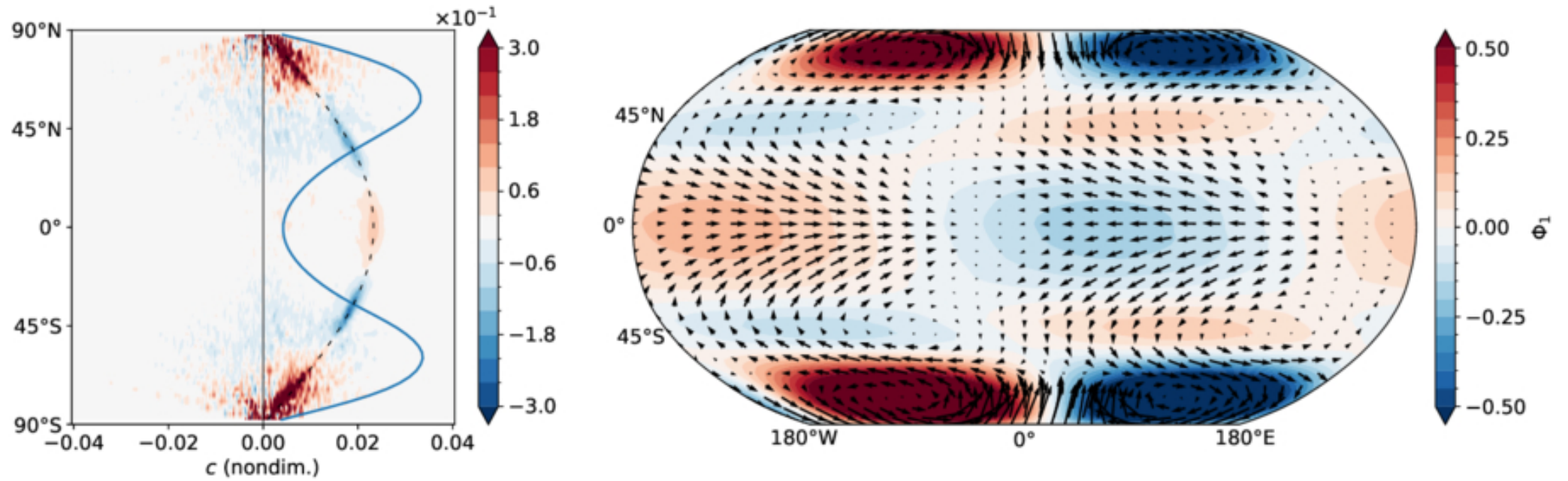
Figure 11. from Quentin Nicolas and Geoffrey K. Vallis 2026 Planet. Sci. J. 7 doi:10.3847/PSJ/ae5c96 https://dx.doi.org/10.3847/PSJ/ae5c96 © 2026. The Author(s). Published by the American Astronomical Society.
