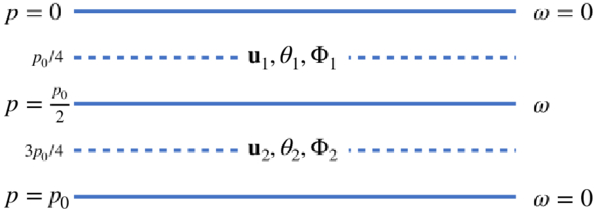
Figure 1. from Quentin Nicolas and Geoffrey K. Vallis 2026 Planet. Sci. J. 7 doi:10.3847/PSJ/ae5c96 https://dx.doi.org/10.3847/PSJ/ae5c96 © 2026. The Author(s). Published by the American Astronomical Society.
