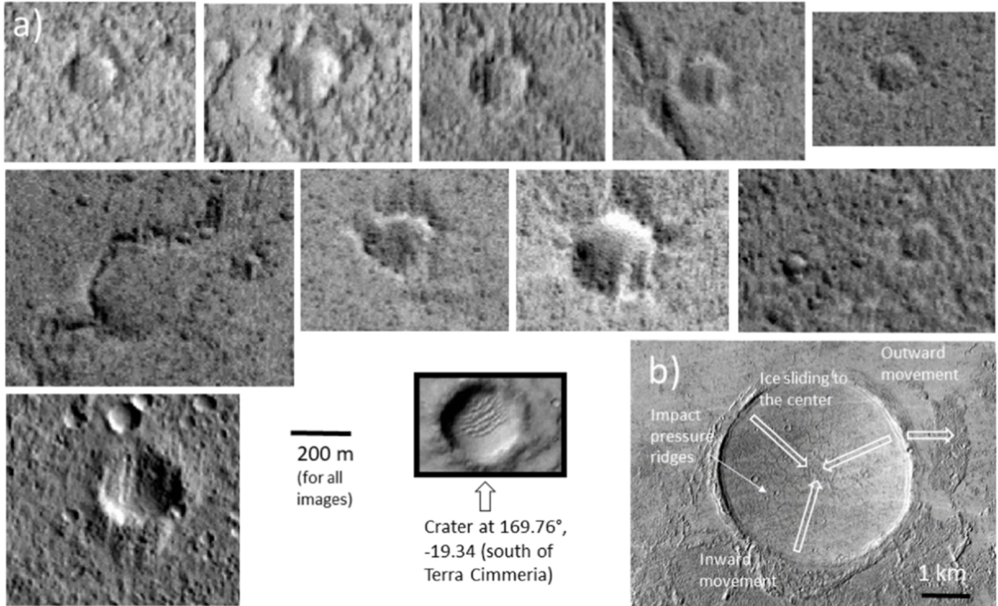
Figure 7. from Fabio Vittorio De Blasio 2026 Planet. Sci. J. 7 doi:10.3847/PSJ/ae5b80 https://dx.doi.org/10.3847/PSJ/ae5b80 © 2026. The Author(s). Published by the American Astronomical Society.
