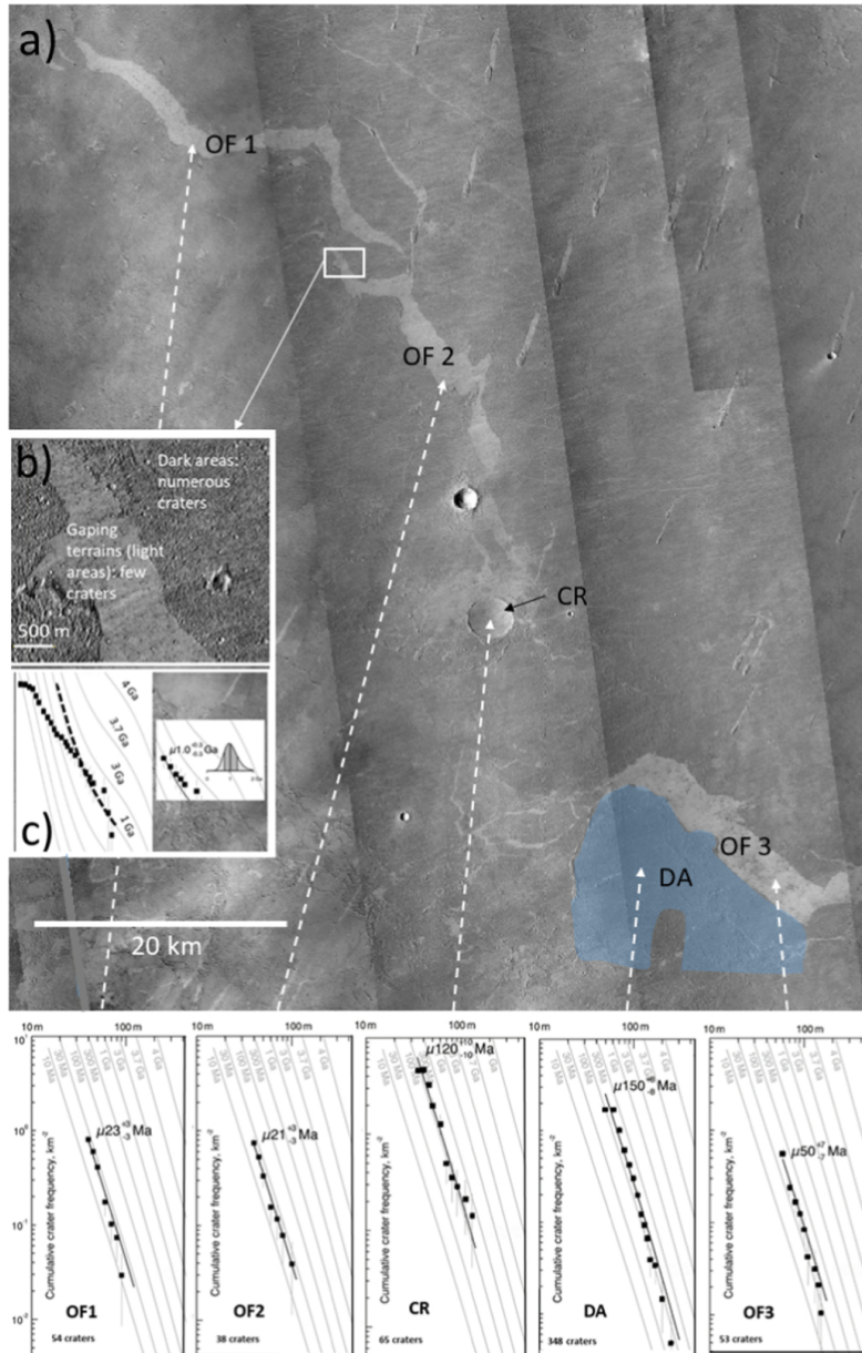
Figure 6. from Fabio Vittorio De Blasio 2026 Planet. Sci. J. 7 doi:10.3847/PSJ/ae5b80 https://dx.doi.org/10.3847/PSJ/ae5b80 © 2026. The Author(s). Published by the American Astronomical Society.
