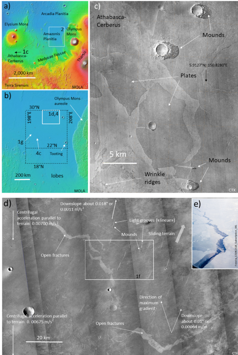
Figure 1. from Fabio Vittorio De Blasio 2026 Planet. Sci. J. 7 doi:10.3847/PSJ/ae5b80 https://dx.doi.org/10.3847/PSJ/ae5b80 © 2026. The Author(s). Published by the American Astronomical Society.
