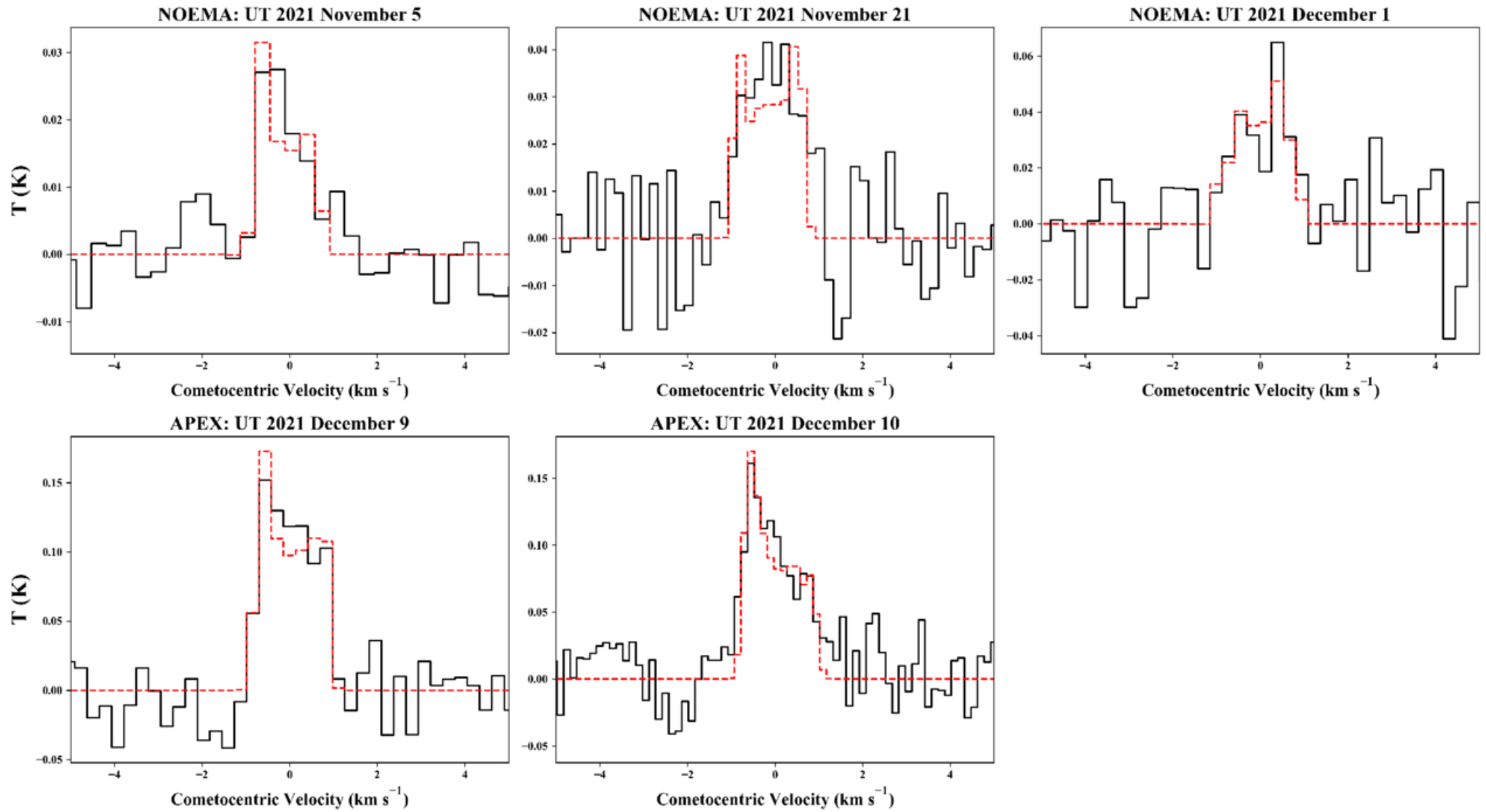
Figure 4. from Timothy N. Proudki et al 2026 Planet. Sci. J. 7 doi:10.3847/PSJ/ae5b73 https://dx.doi.org/10.3847/PSJ/ae5b73 © 2026. The Author(s). Published by the American Astronomical Society.
