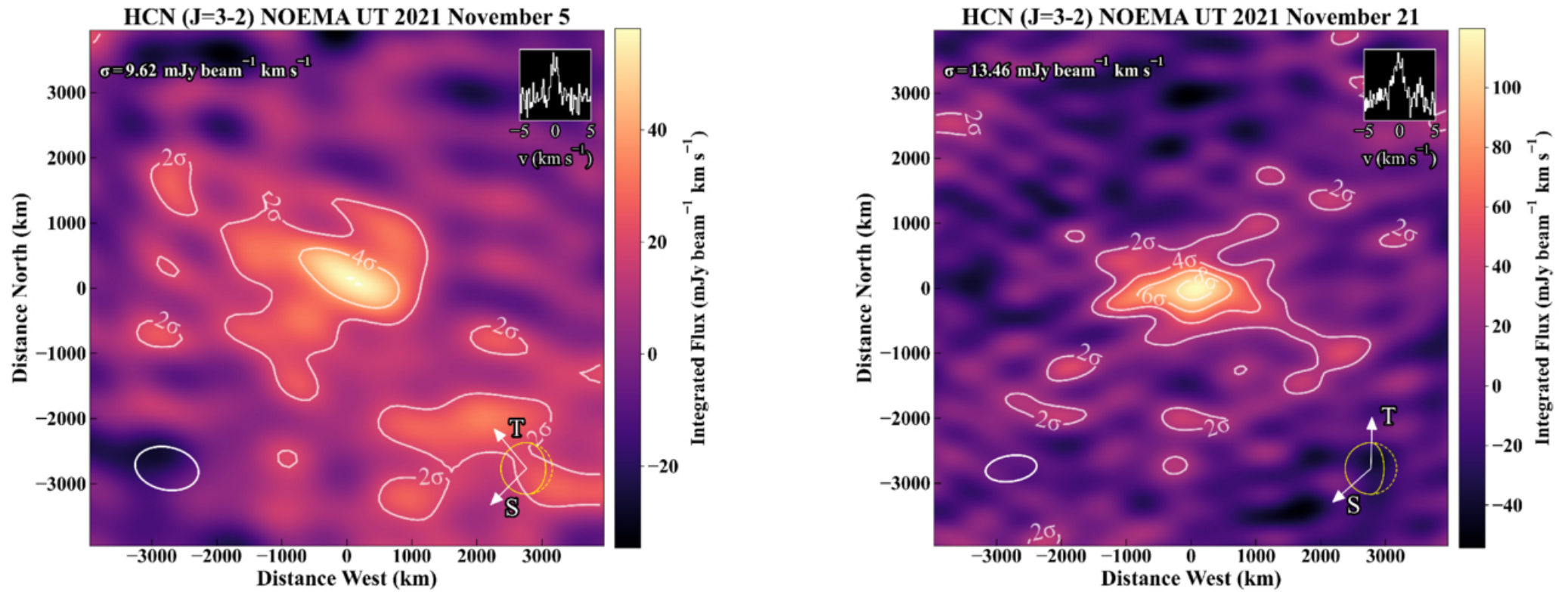
Figure 1. from Timothy N. Proudki et al 2026 Planet. Sci. J. 7 doi:10.3847/PSJ/ae5b73 https://dx.doi.org/10.3847/PSJ/ae5b73 © 2026. The Author(s). Published by the American Astronomical Society.
